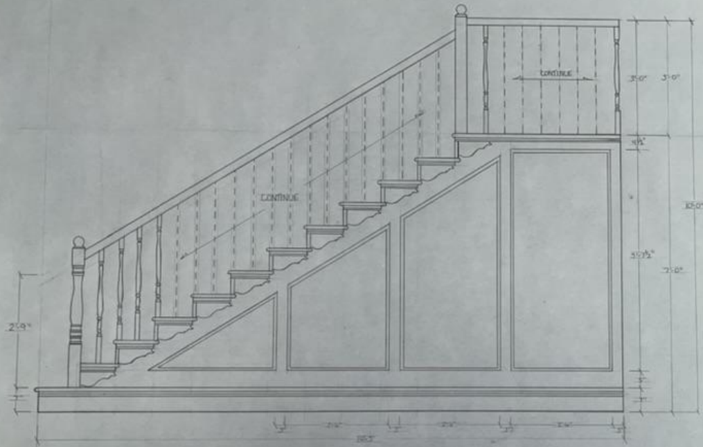
FRONT ELEVATION
