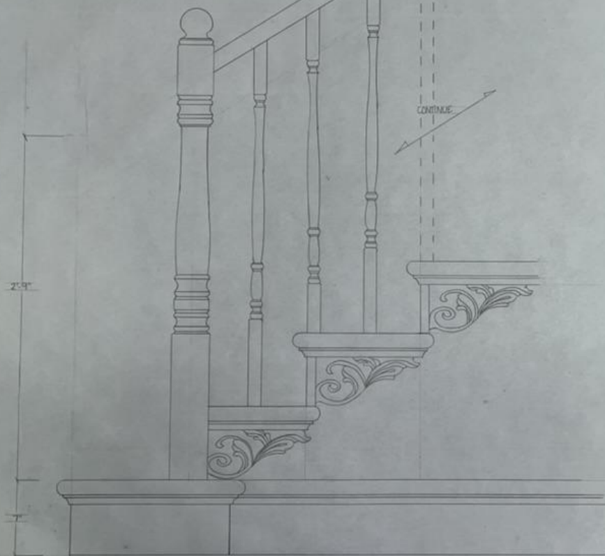
BALUSTRADE DETAIL SCALE 3/4"=1'-0"
