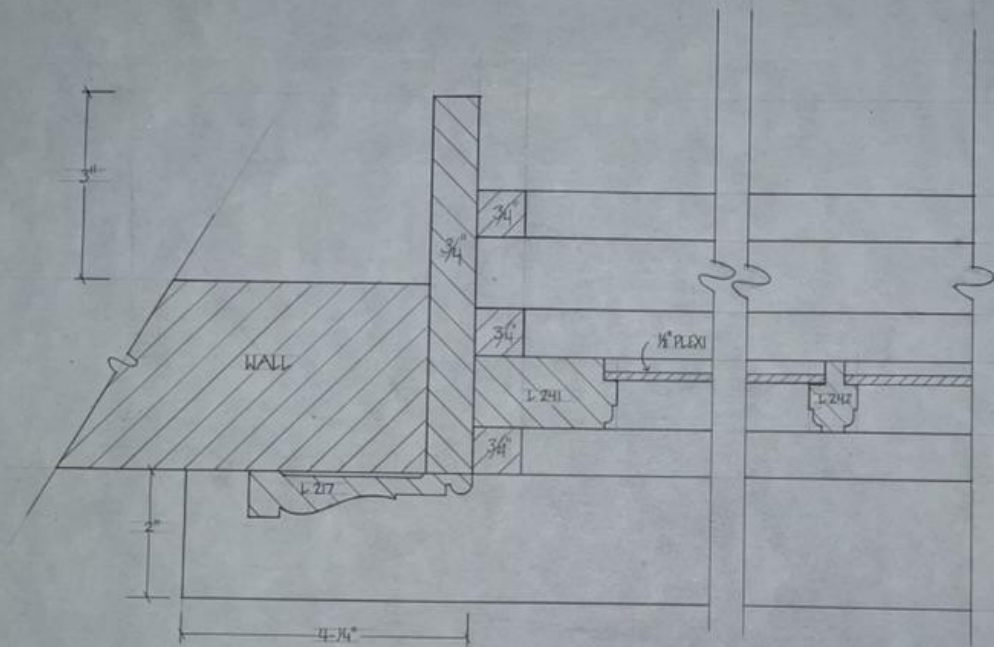
WINDOW DETAIL 2 SCALE: FULL SIZE
