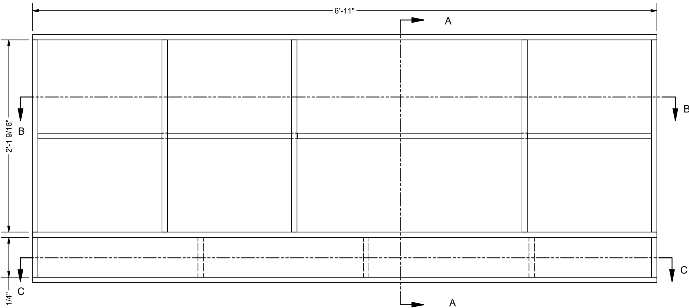
200995-02-D CENTER BOOKSHELF SCALE 1 1/2" = 1'-0"
