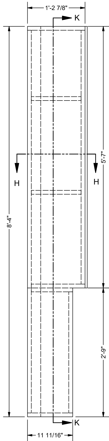
200995-01-C SCALE 1" = 1'-0"
