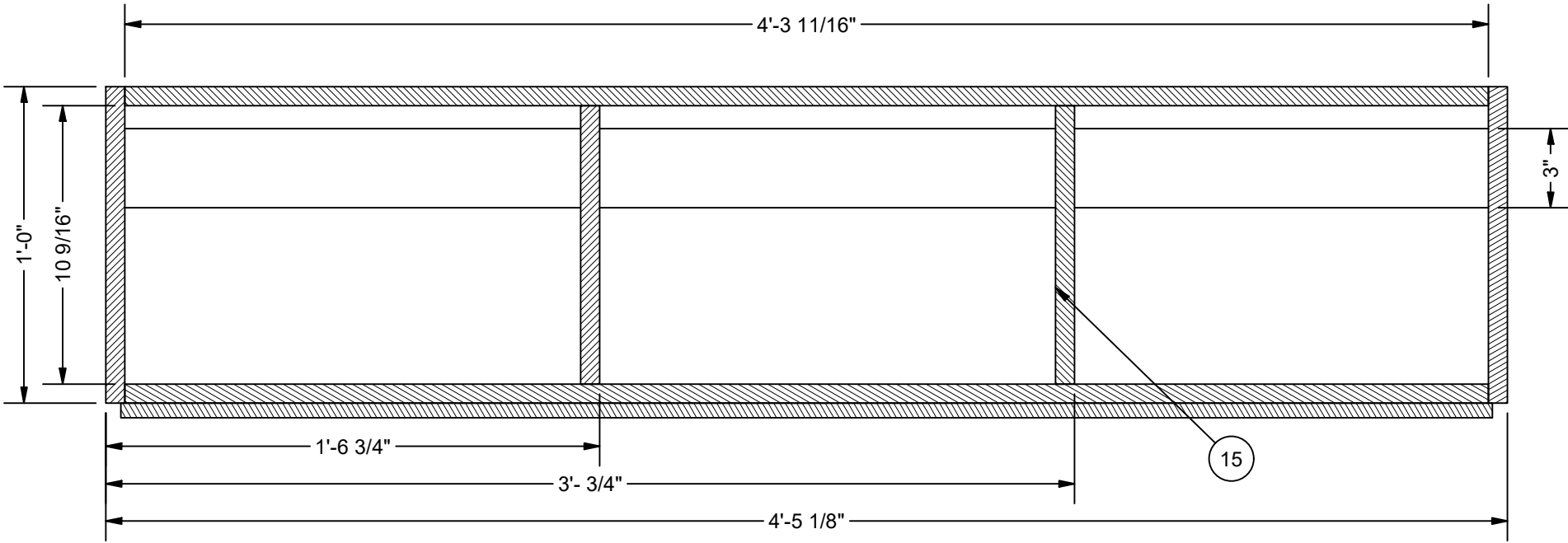
SECTION J-J SCALE 2" = 1'-0"
