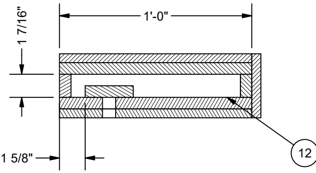
SECTION I-I SCALE 2" = 1'-0"
