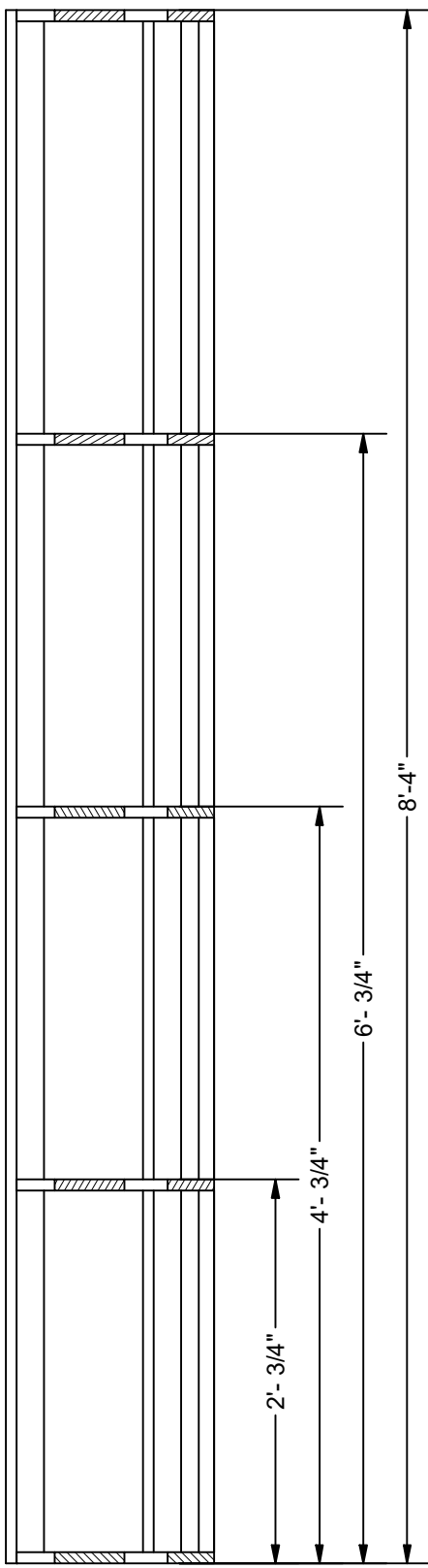
SECTION A-A SCALE 1" = 1'-0"
