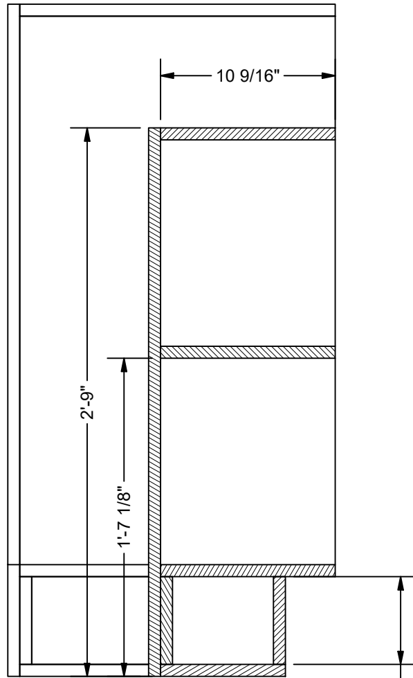
SECTION B-B SCALE 1 1/2" = 1'-0"
