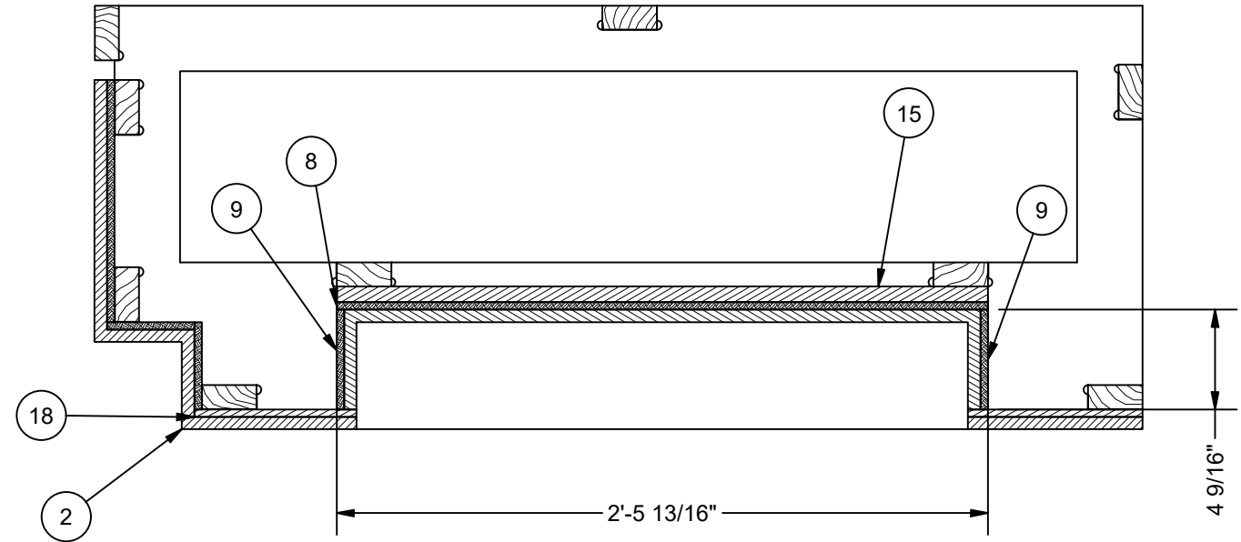
SECTION B-B SCALE 1 1/2" = 1'-0"
