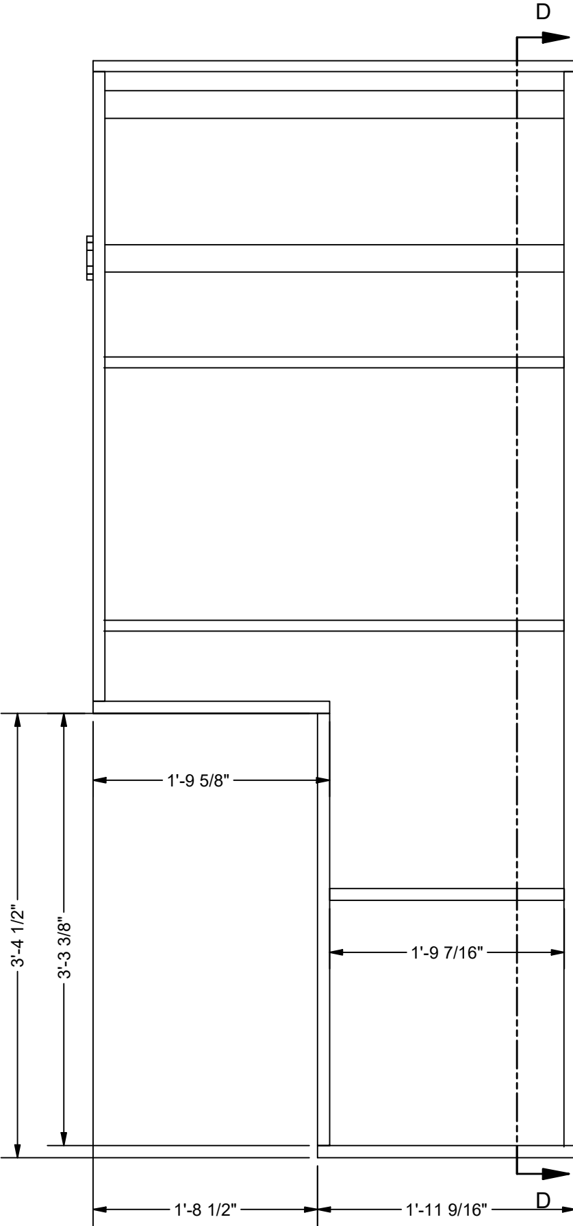
200995-01-A SCALE 1" = 1'-0"
