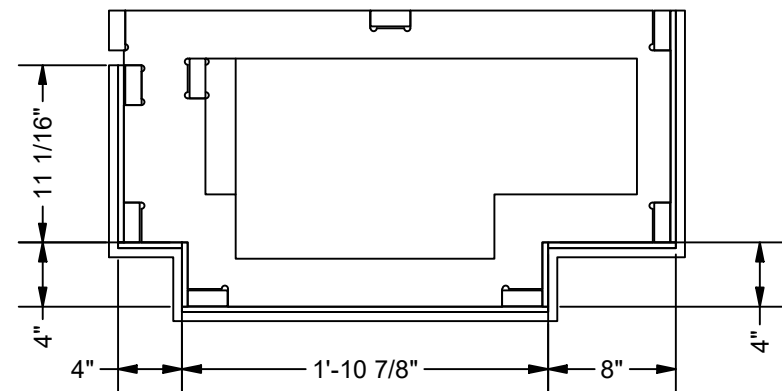
TOP SCALE 1" = 1'-0"
