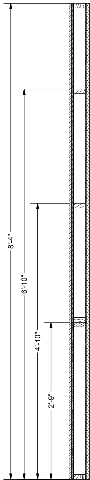
SECTION K-K SCALE 1" = 1'-0"
