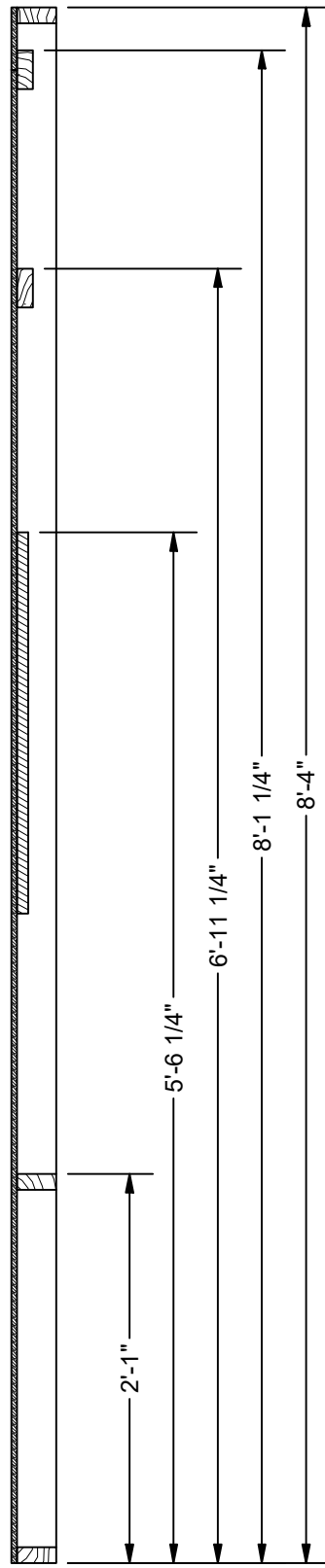
SECTION C-C SCALE 1" = 1'-0"
