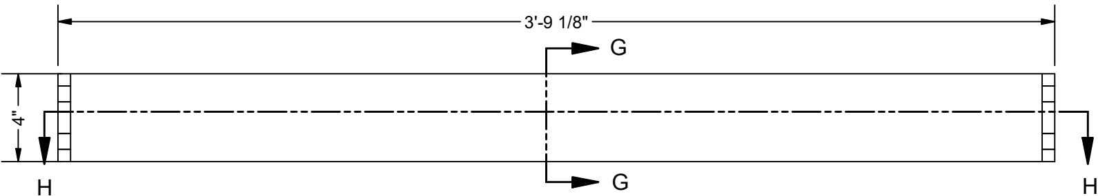
LEFT FLOATING SHELF SCALE 2" = 1'-0"
