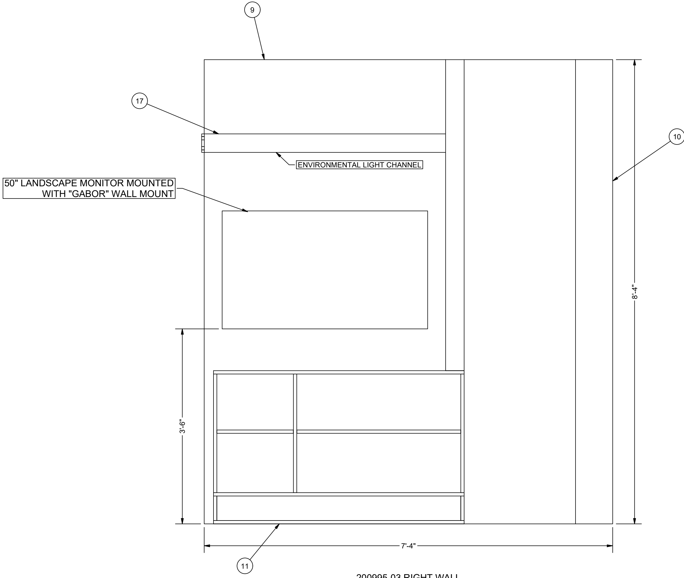
200995-03 RIGHT WALL SCALE 1" = 1'-0"
