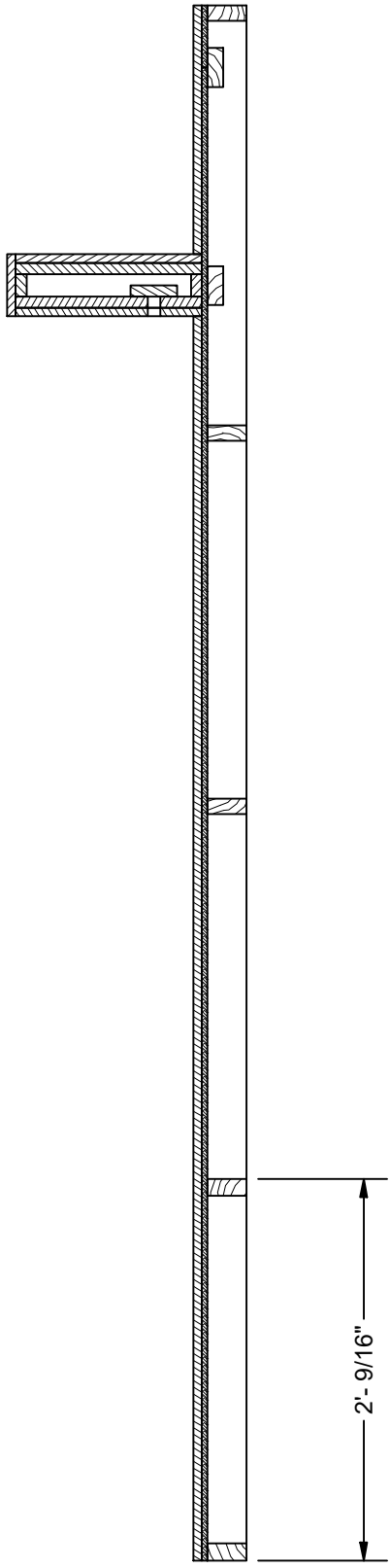
SECTION D-D SCALE 1" = 1'-0"
