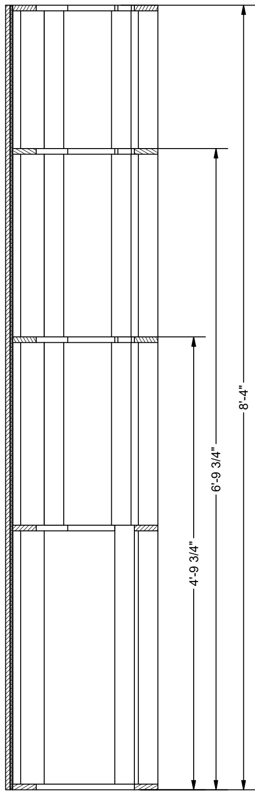
SECTION G-G SCALE 1" = 1'-0"
