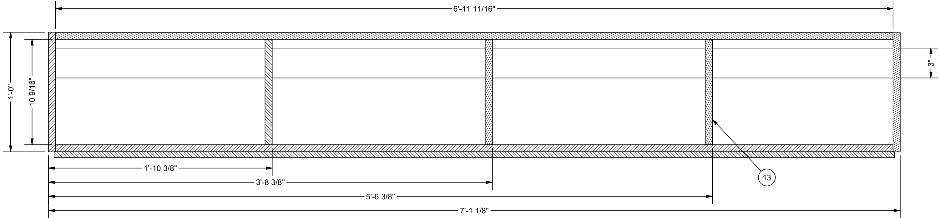
SECTION L-L SCALE 2" = 1'-0"
