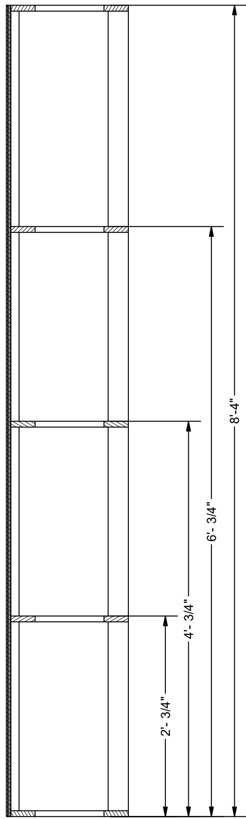
SECTION B-B SCALE 1" = 1'-0"
