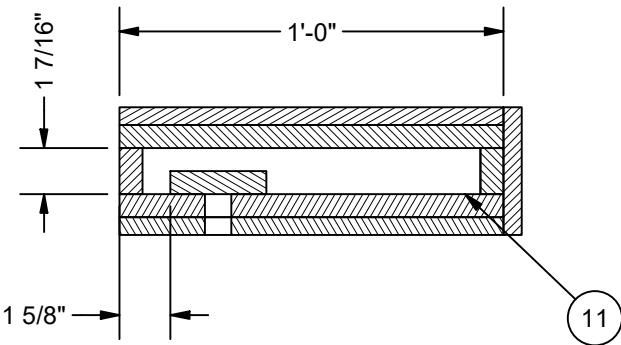
SECTION G-G SCALE 2" = 1'-0"
