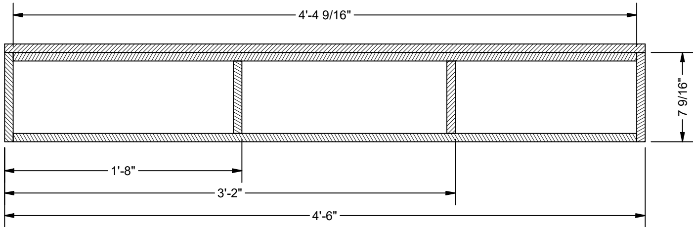
SECTION F-F SCALE 1 1/2" = 1'-0"
