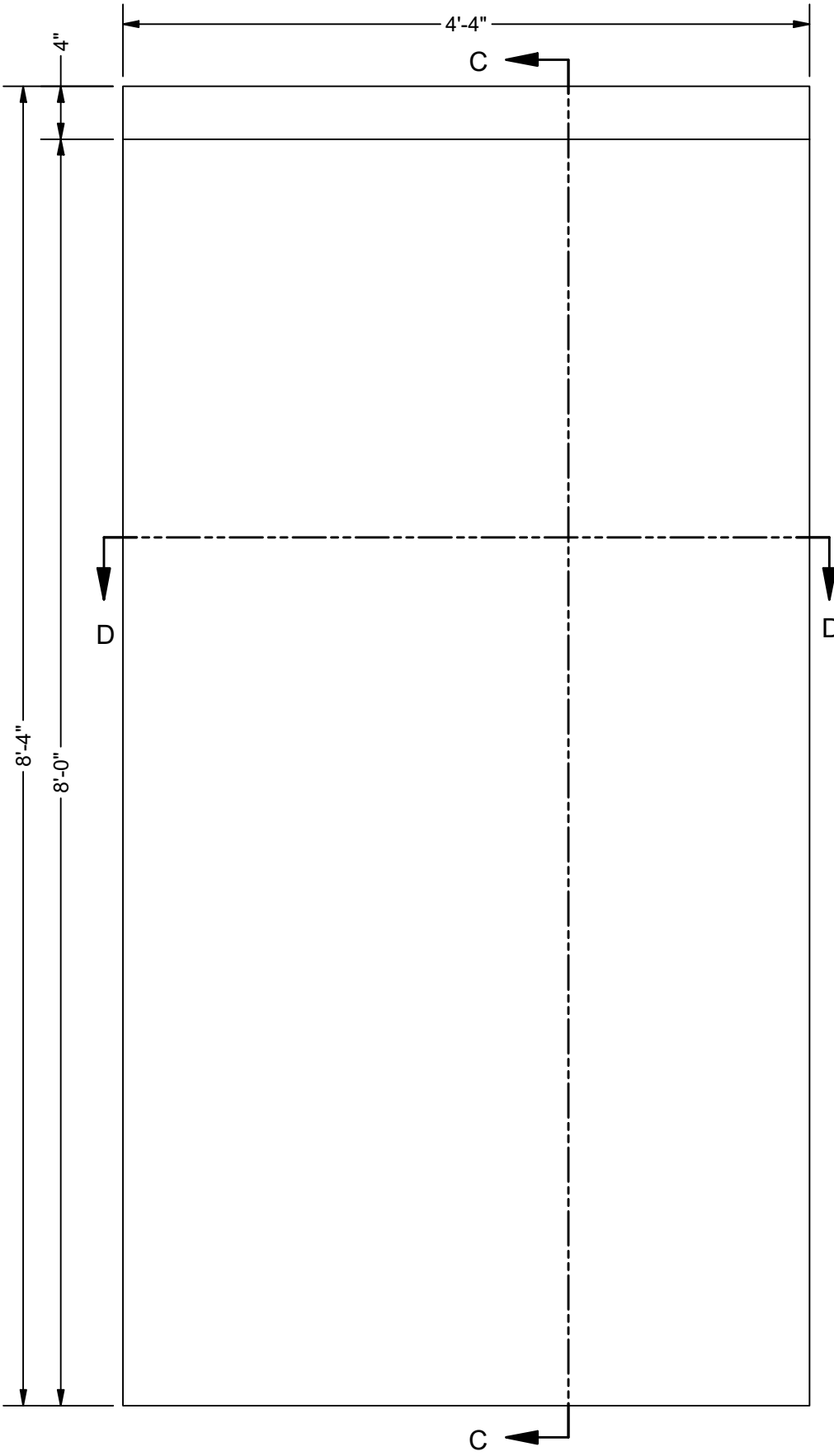
RIGHT WALL-A SCALE 1" = 1'-0"
