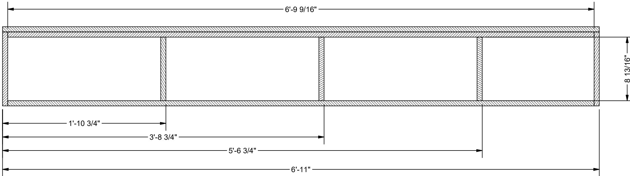
SECTION C-C SCALE 1 1/2" = 1'-0"
