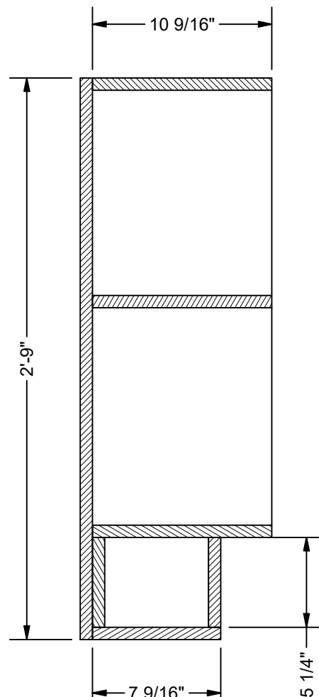
SECTION D-D SCALE 1 1/2" = 1'-0"
