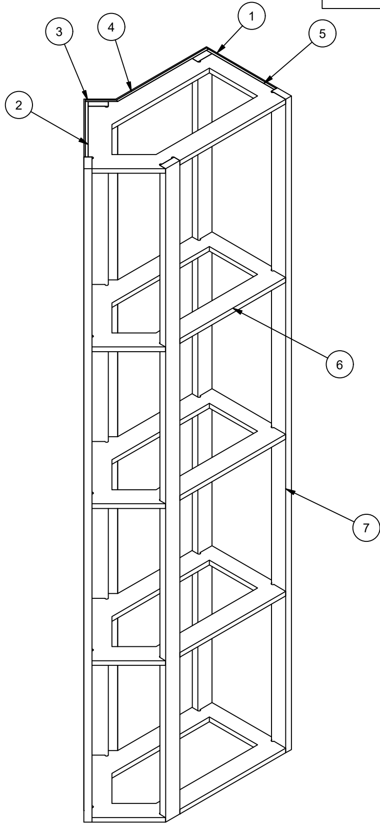
200995-02-C SCALE 1" = 1'-0"
