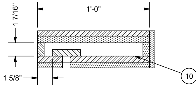
SECTION K-K SCALE 2" = 1'-0"
