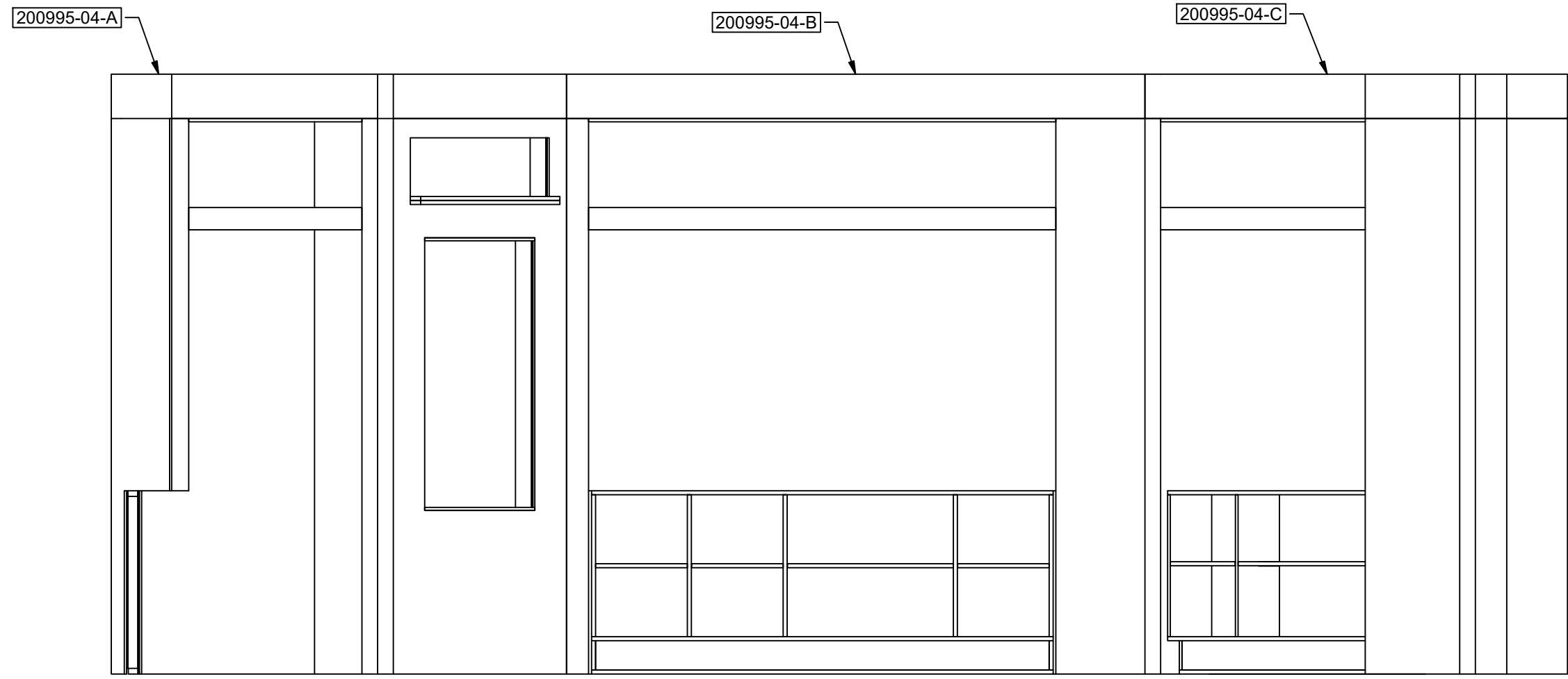
200995 MASTER ASSEMBLY SCALE 1/2" = 1'-0"
