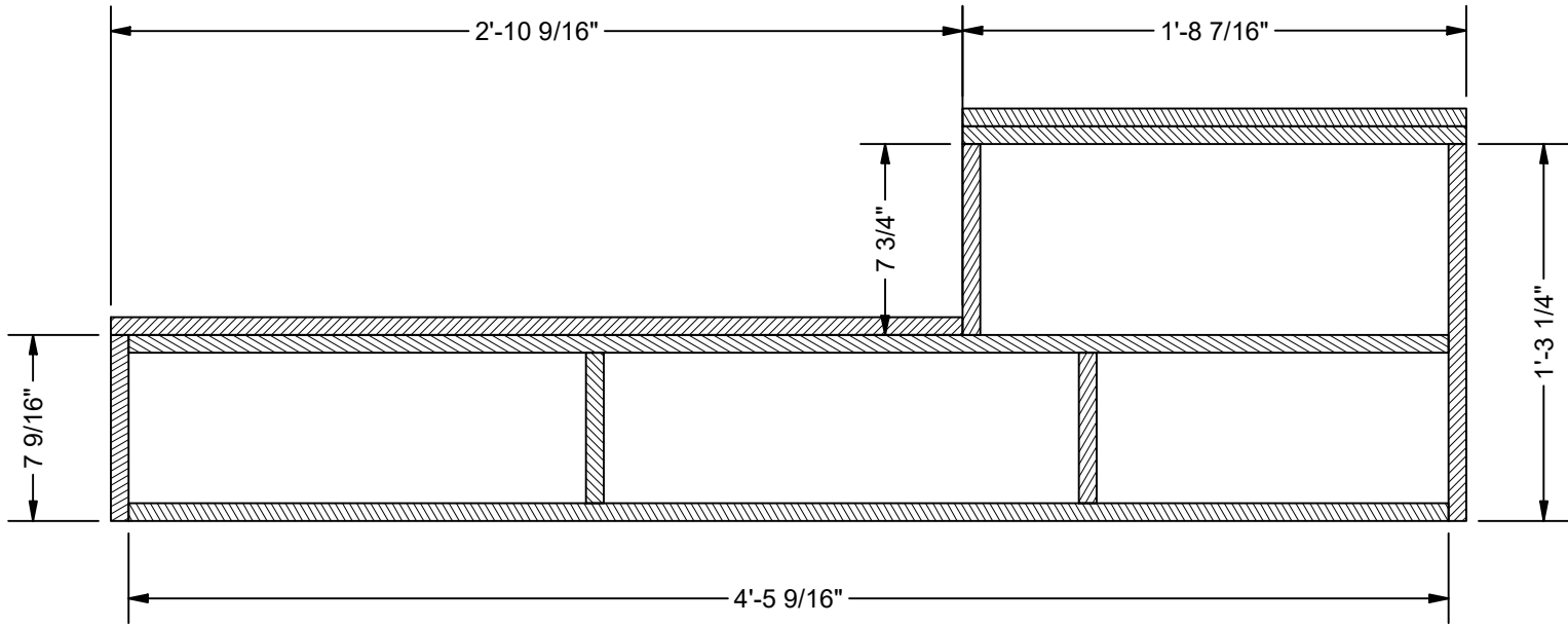
SECTION A-A SCALE 1 1/2" = 1'-0"
