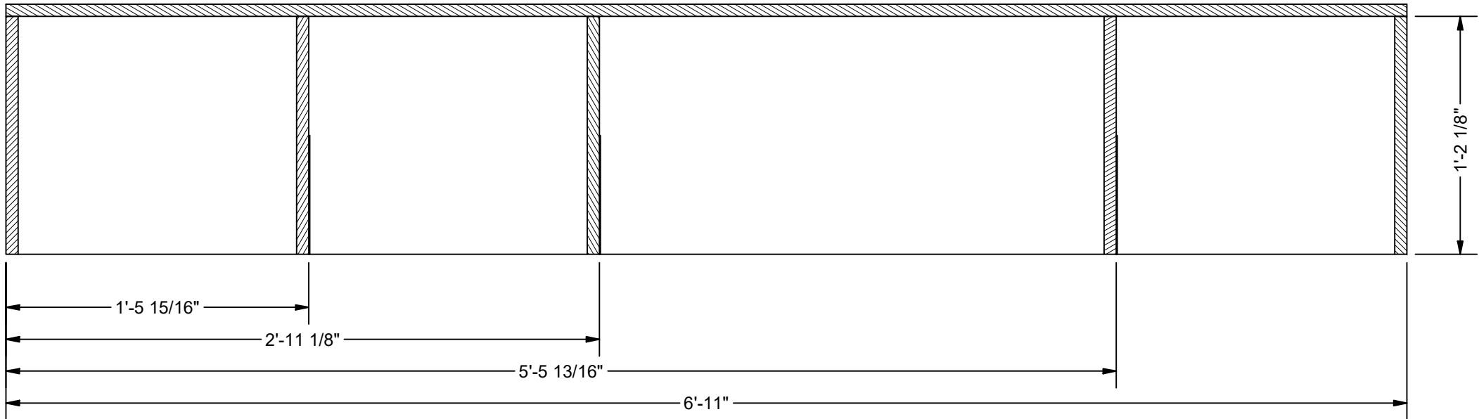
SECTION B-B SCALE 1 1/2" = 1'-0"
