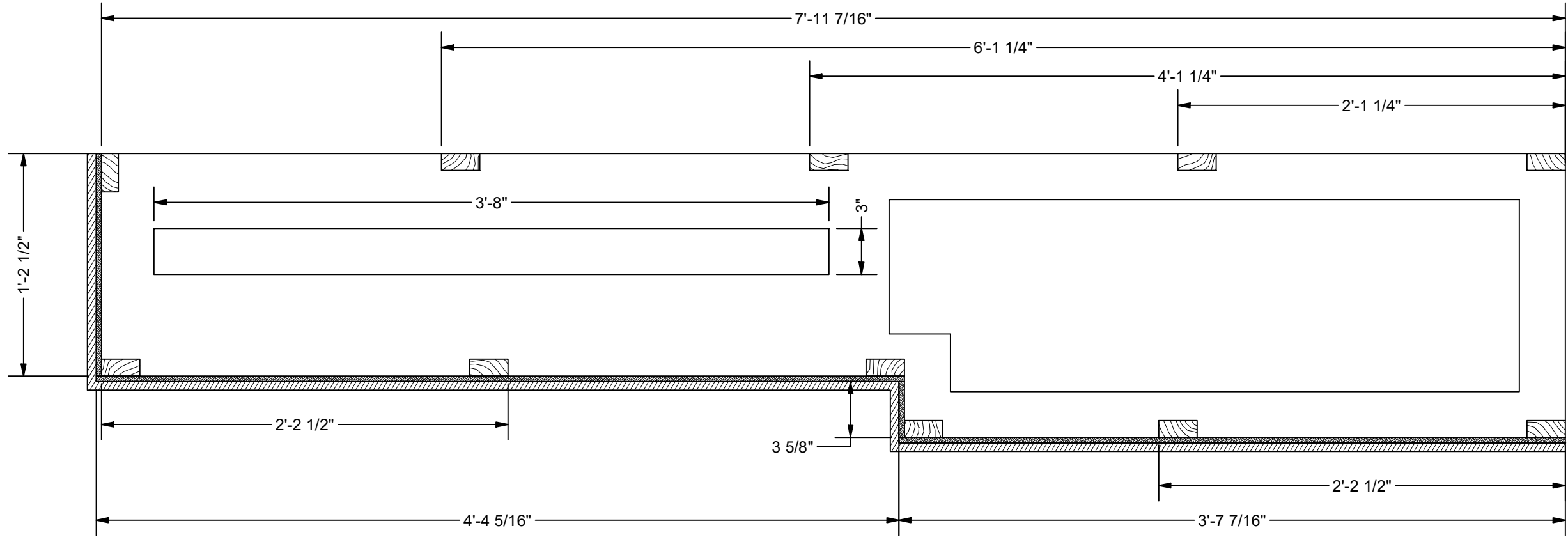
SECTION A-A SCALE 1 1/2" = 1'-0"
