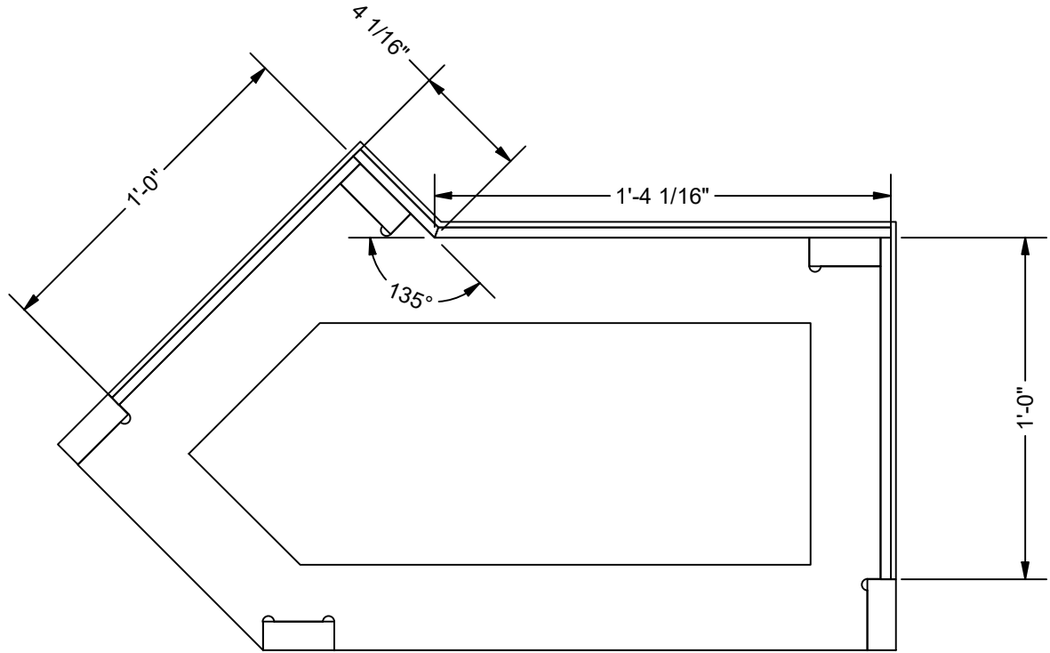
TOP SCALE 2" = 1'-0"
