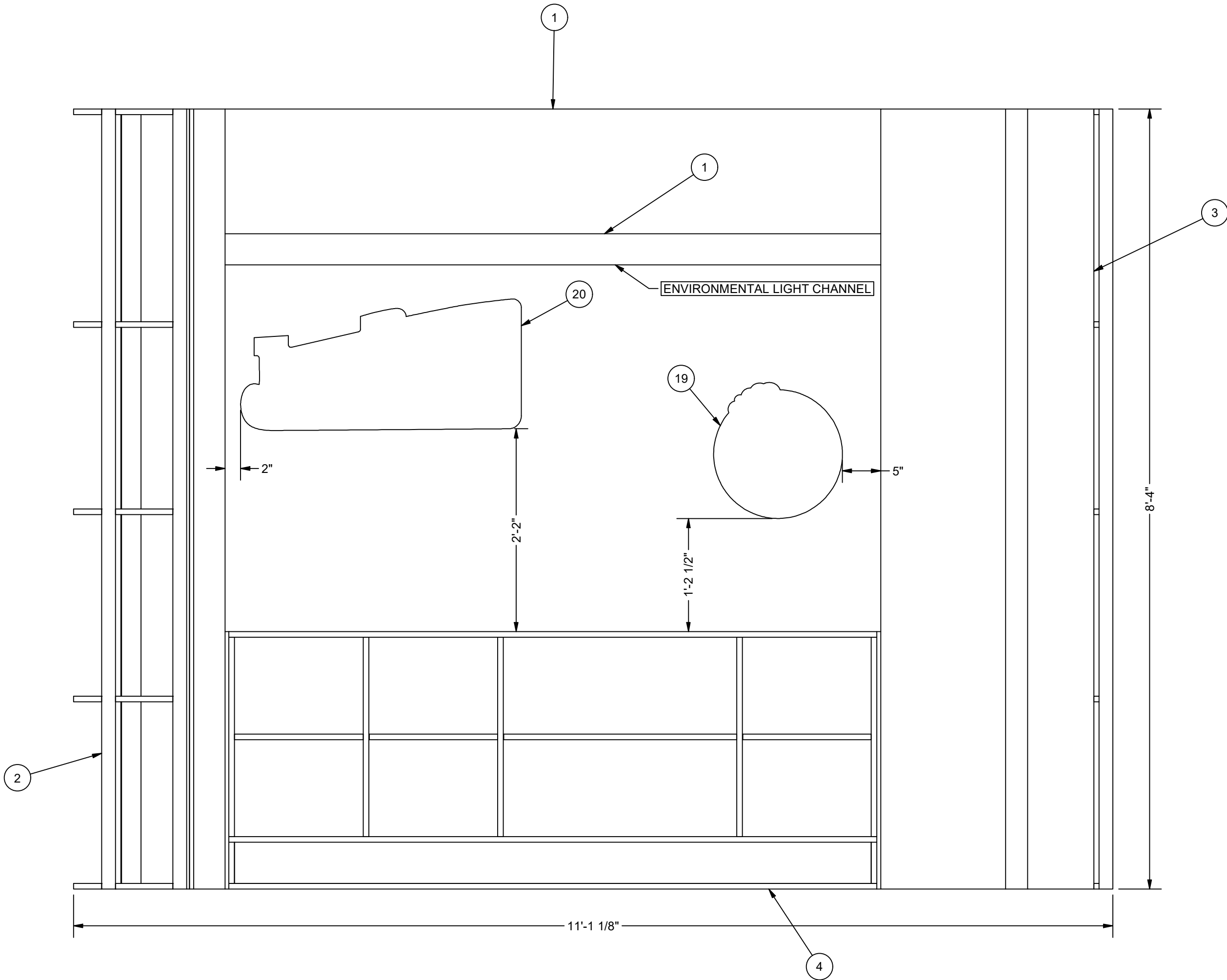
200995-02 CENTER WALL SCALE 1" = 1'-0"
