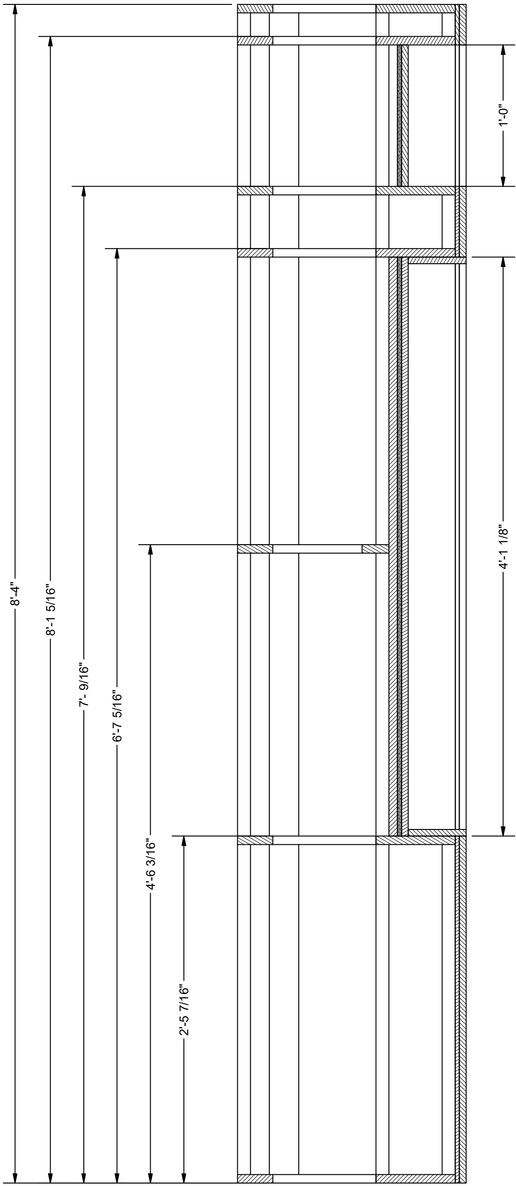
SECTION A-A SCALE 1 1/2" = 1'-0"
