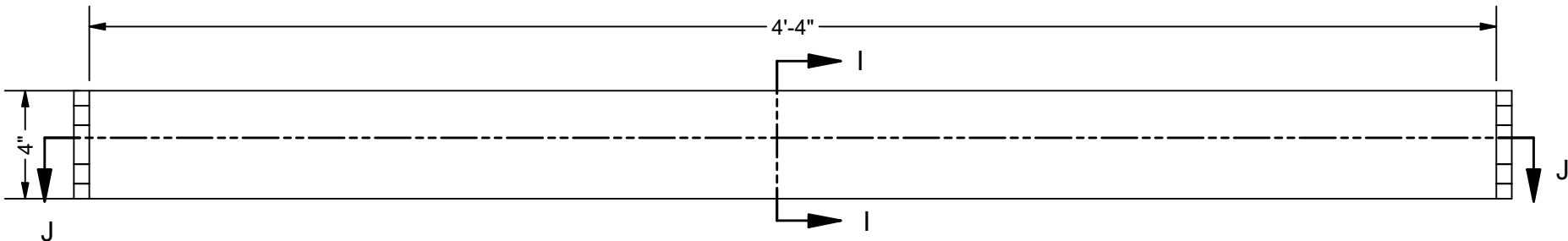
RIGHT FLOATING SHELF SCALE 2" = 1'-0"
