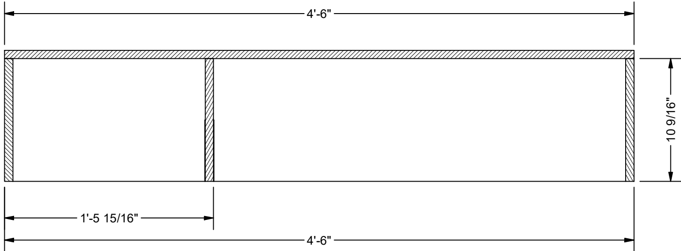
SECTION E-E SCALE 1 1/2" = 1'-0"
