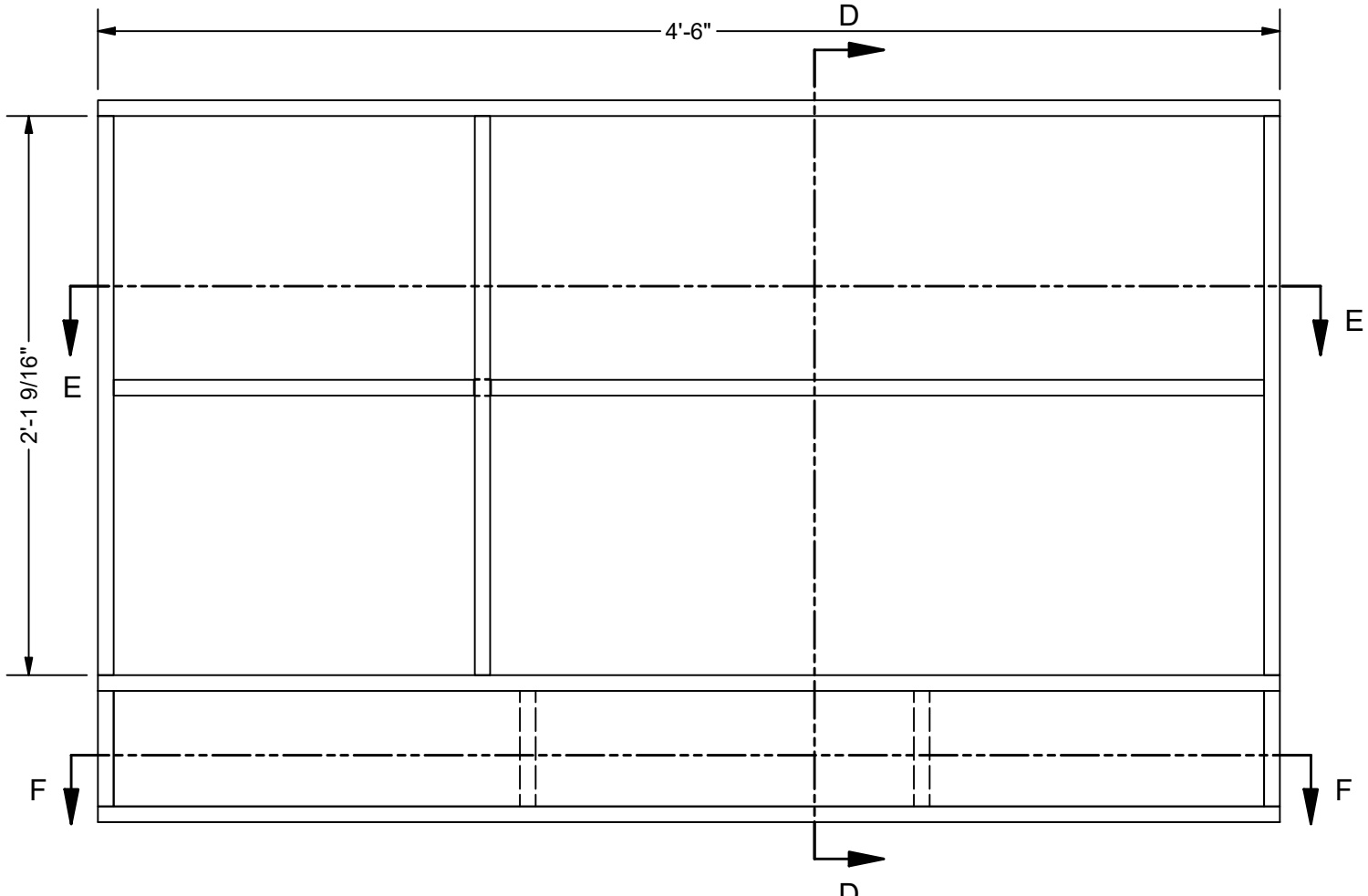
200995-03-C RIGHT BOOKSHELF SCALE 1 1/2" = 1'-0"
