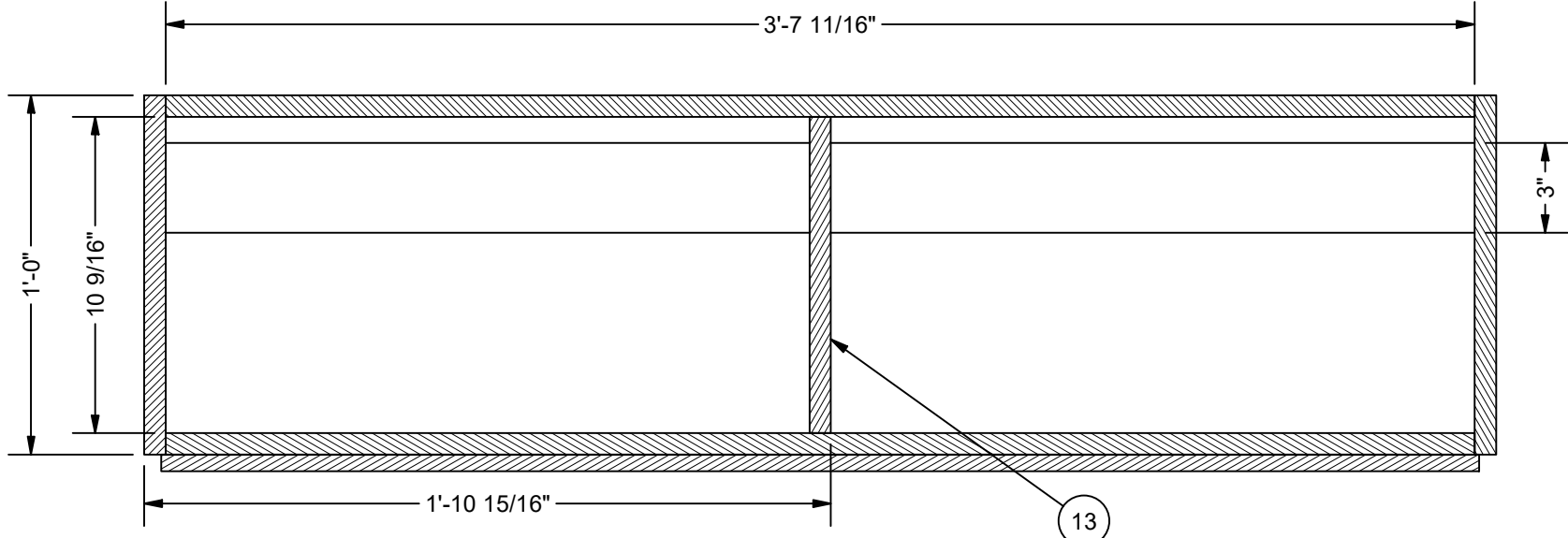
SECTION H-H SCALE 2" = 1'-0"
