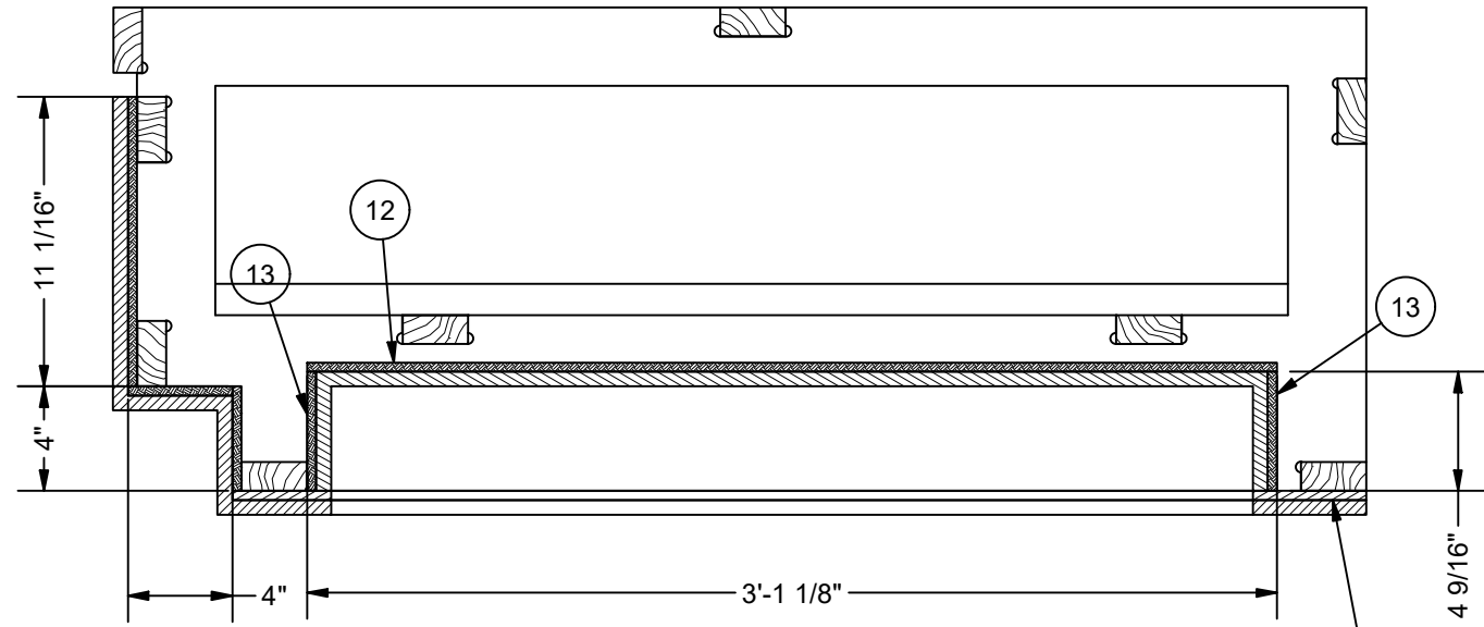
SECTION C-C SCALE 1 1/2" = 1'-0"
