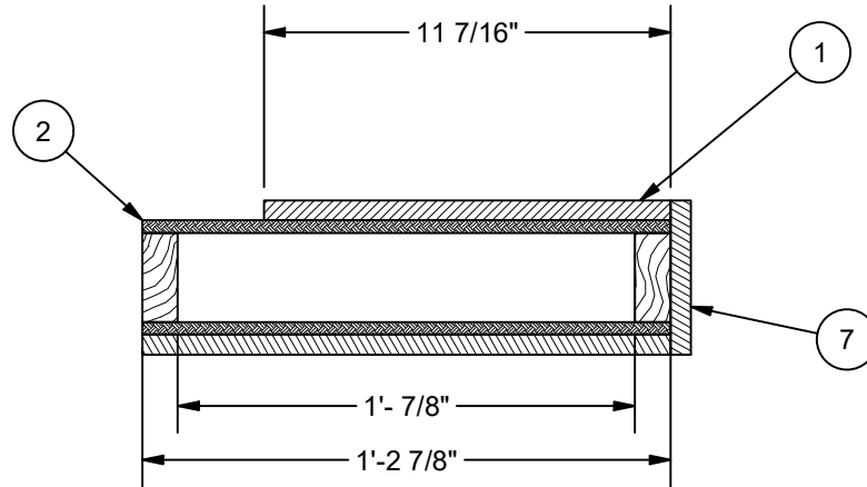
SECTION H-H SCALE 2" = 1'-0"
