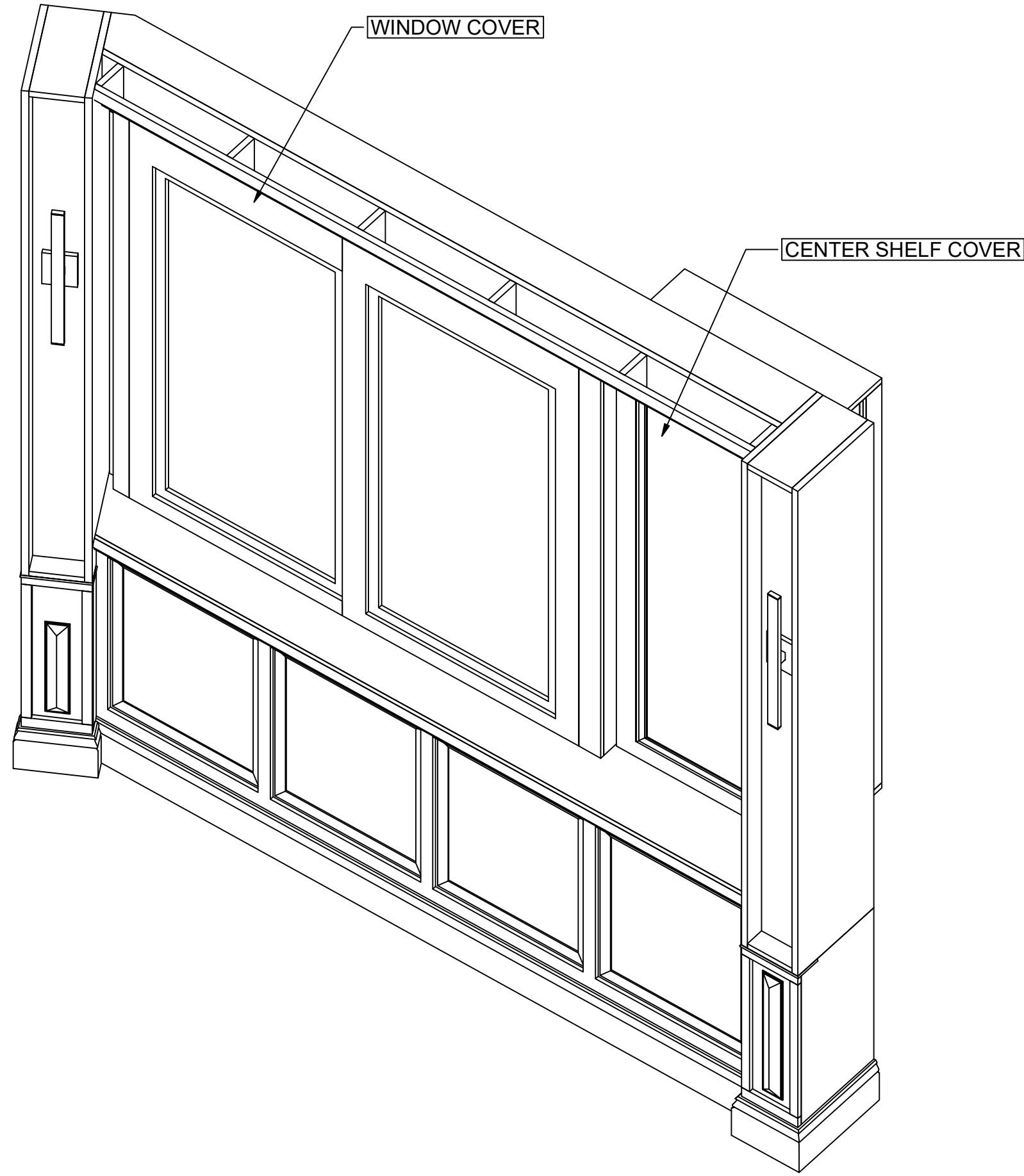
WINDOW WALL ISO SCALE 1" = 1'-0"
