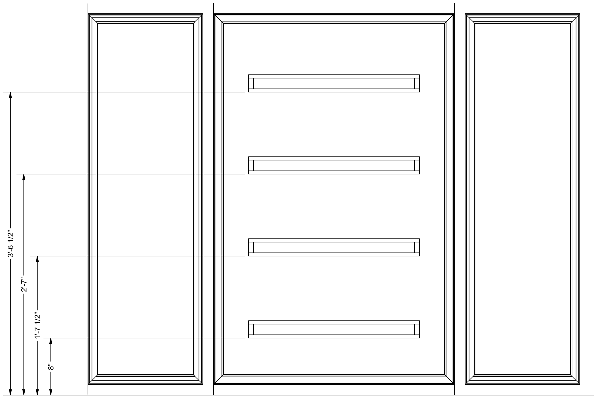
RIGHT SHELF PLACEMENT SCALE 1 1/2" = 1'-0"
