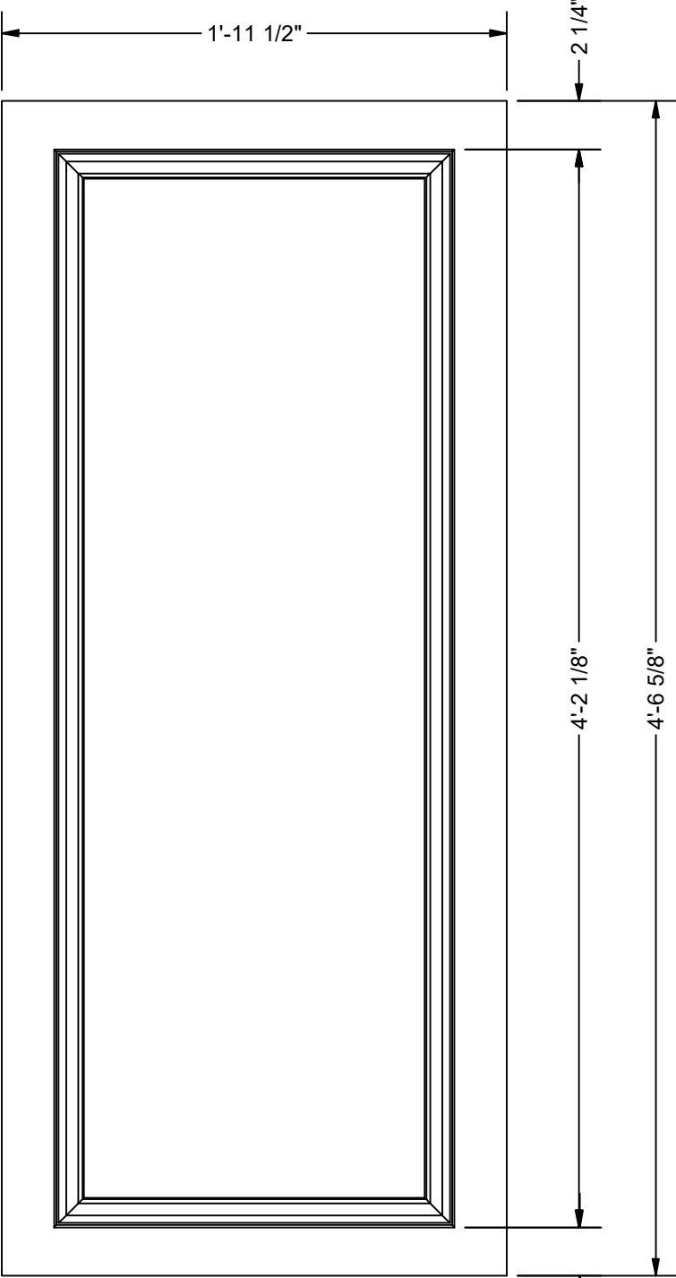
CENTER SHELF COVER FRONT SCALE 1 1/2" = 1'-0"
