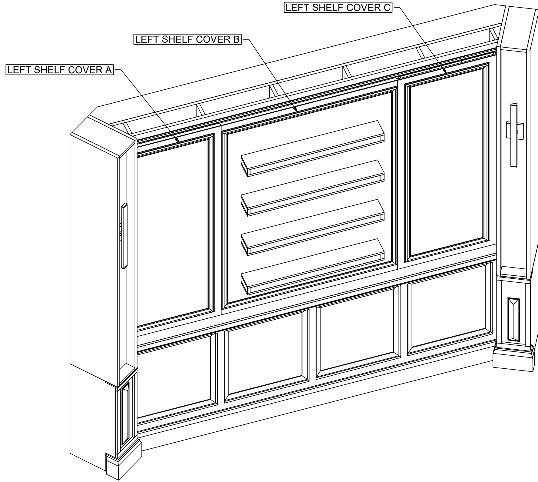
LEFT WALL ISO SCALE 1" = 1'-0"
