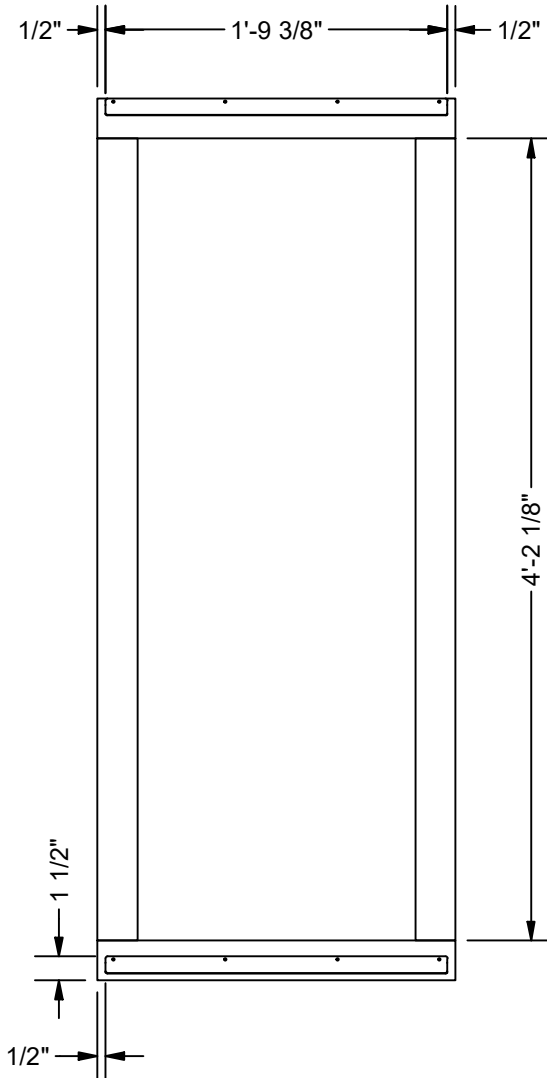
LEFT SHELF COVER C BACK VIEW SCALE 1" = 1'-0"
