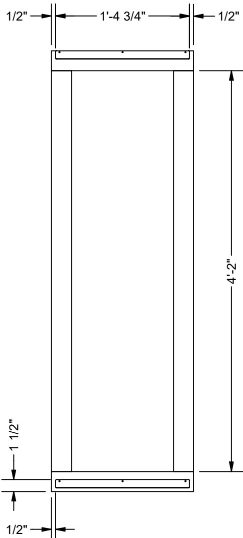
RIGHT SHELF COVER A BACK SCALE 1" = 1'-0"
