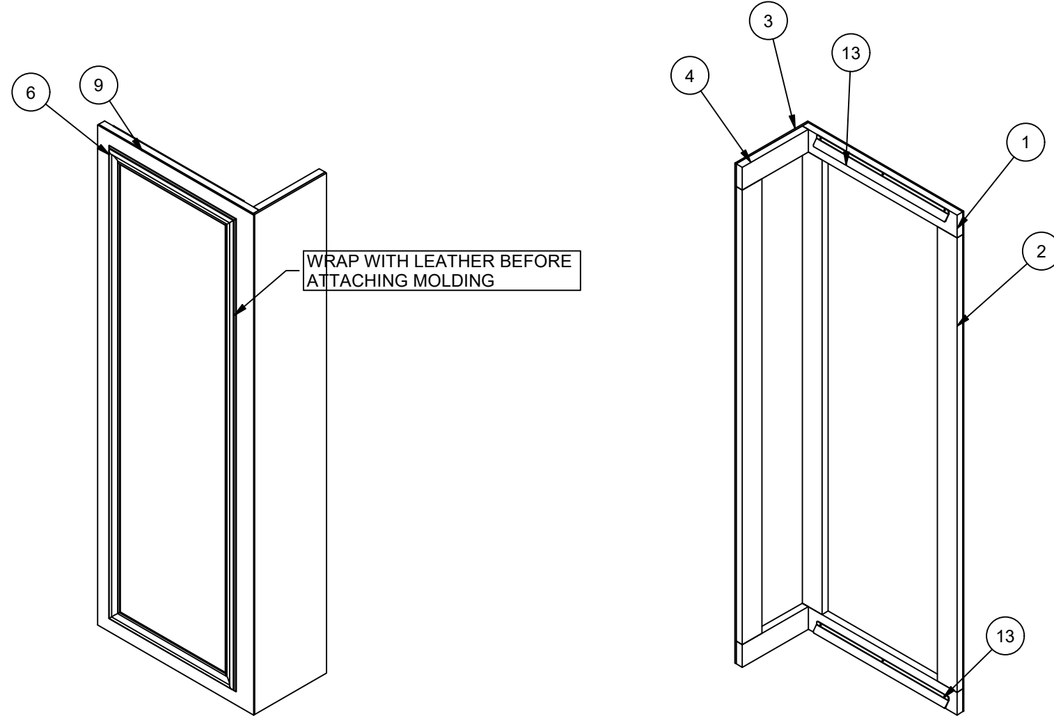
RIGHT SHELF COVER C FRONT ISO SCALE 1" = 1'-0"
