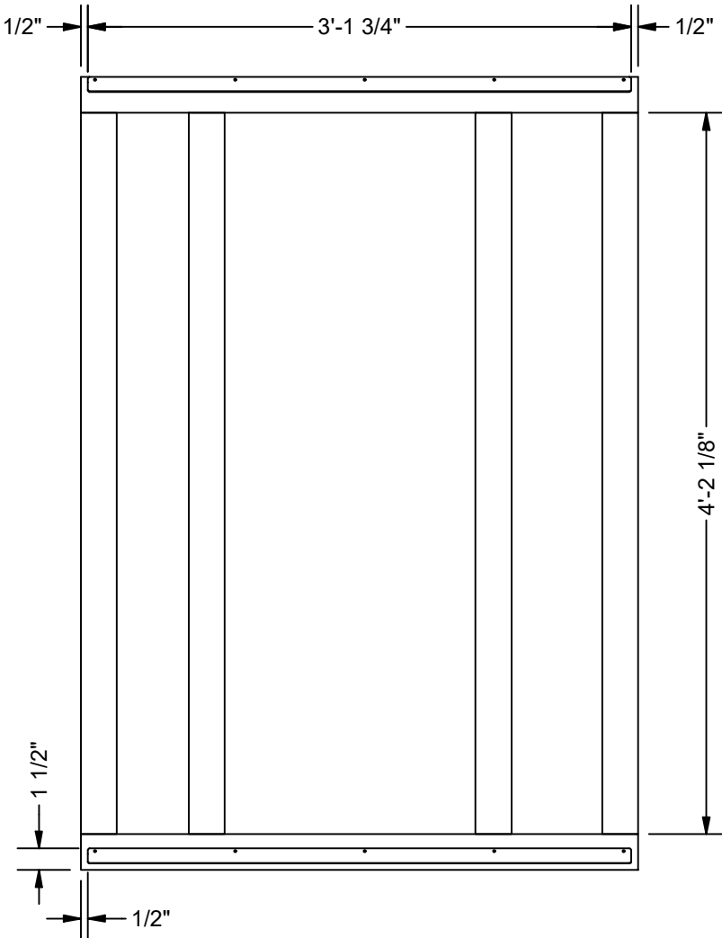
LEFT SHELF COVER B BACK VIEW SCALE 1" = 1'-0"
