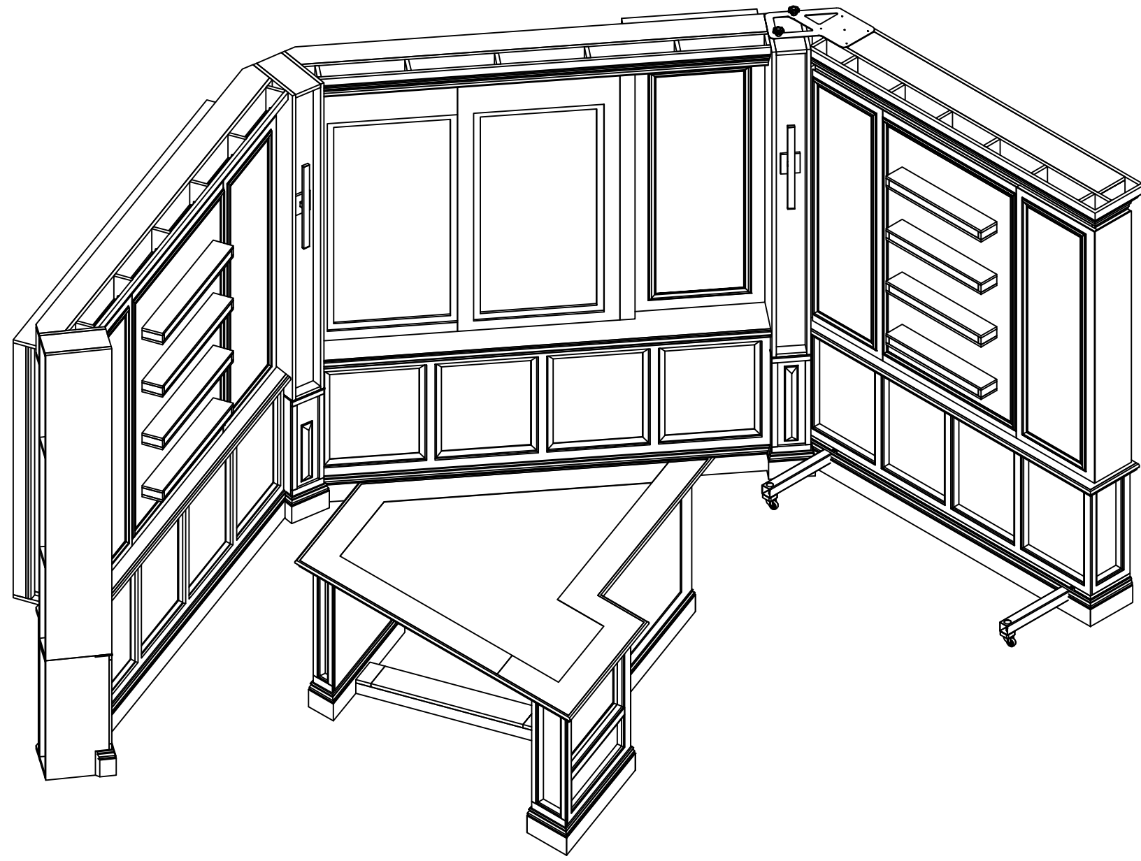
200909-MASTER ASSEMBLY SCALE 1/2" = 1'-0"
