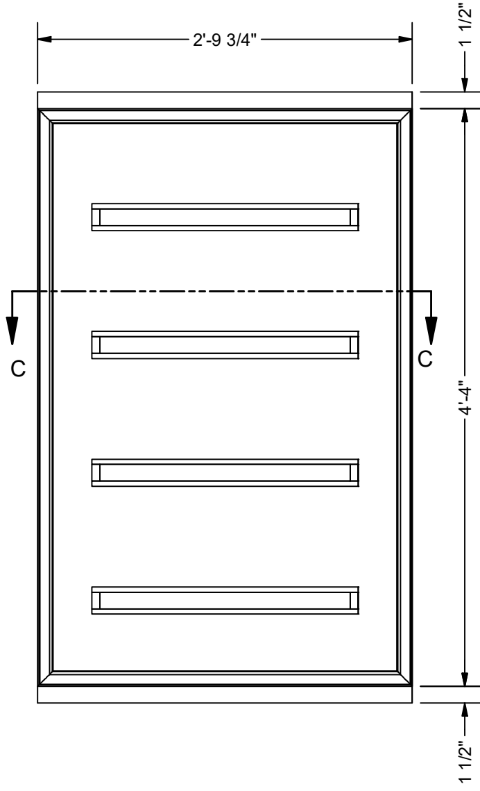
RIGHT SHELF COVER B FRONT SCALE 1" = 1'-0"
