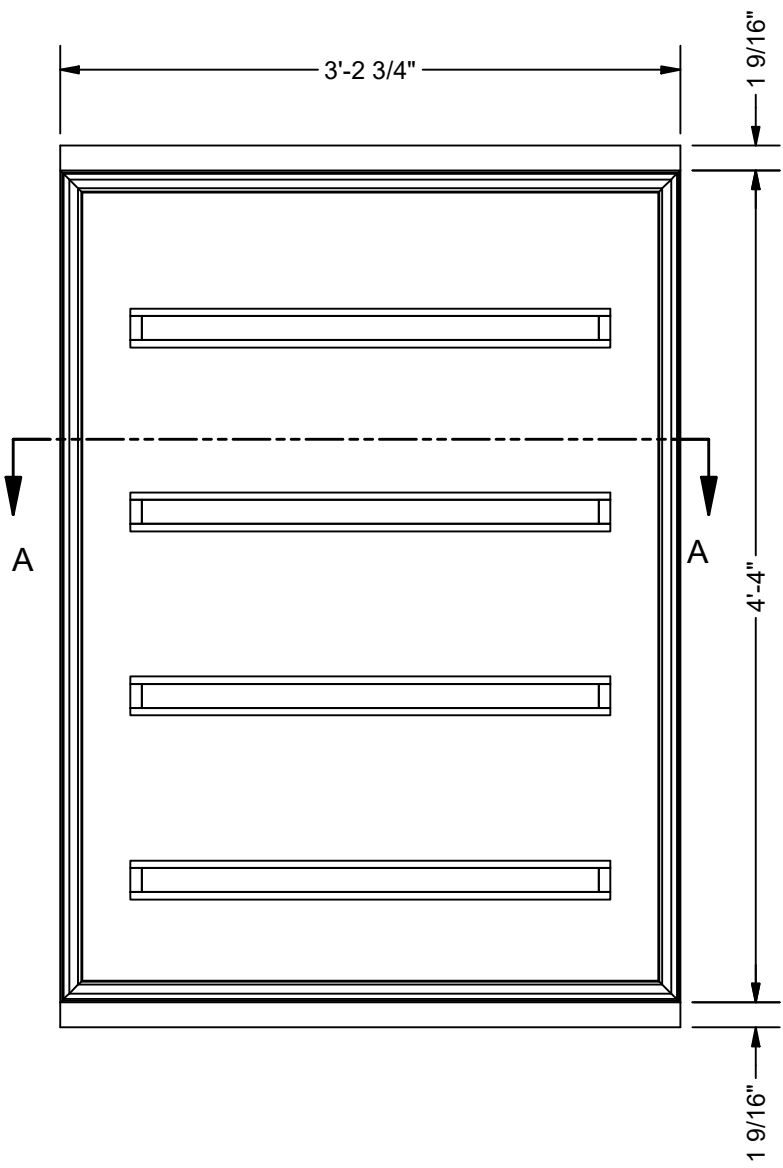
LEFT SHELF COVER B FRONT VIEW SCALE 1" = 1'-0"
