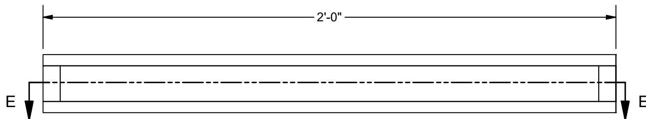
RIGHT FLOATING SHELF FRONT SCALE 3" = 1'-0"
