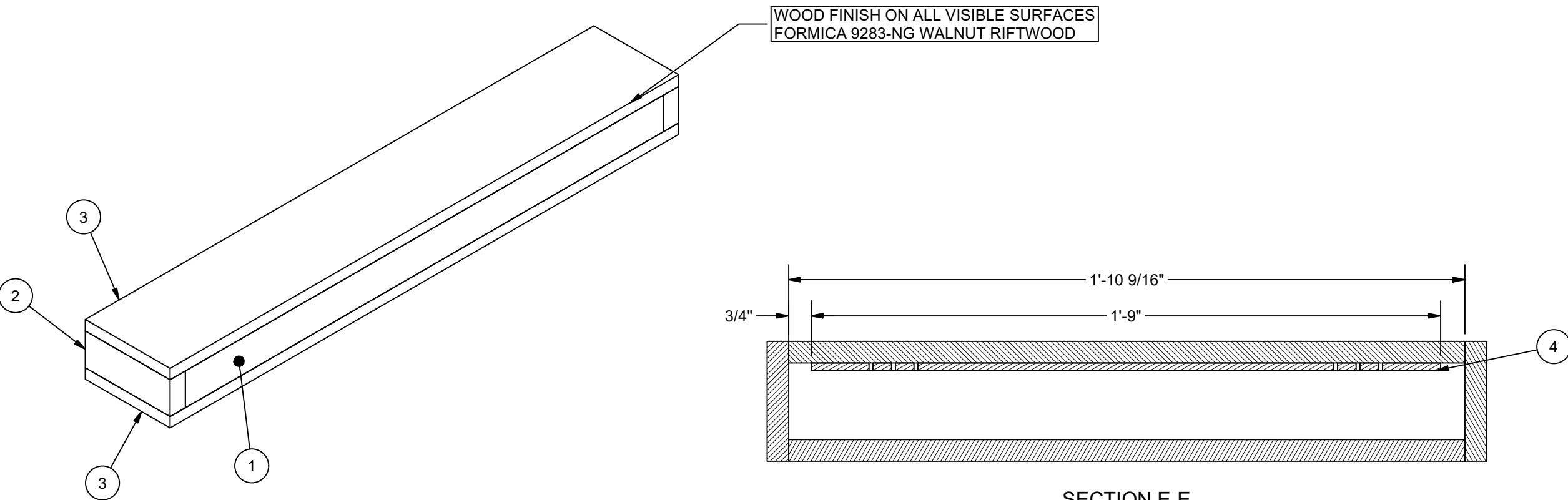
SECTION E-E SCALE 3" = 1'-0"
