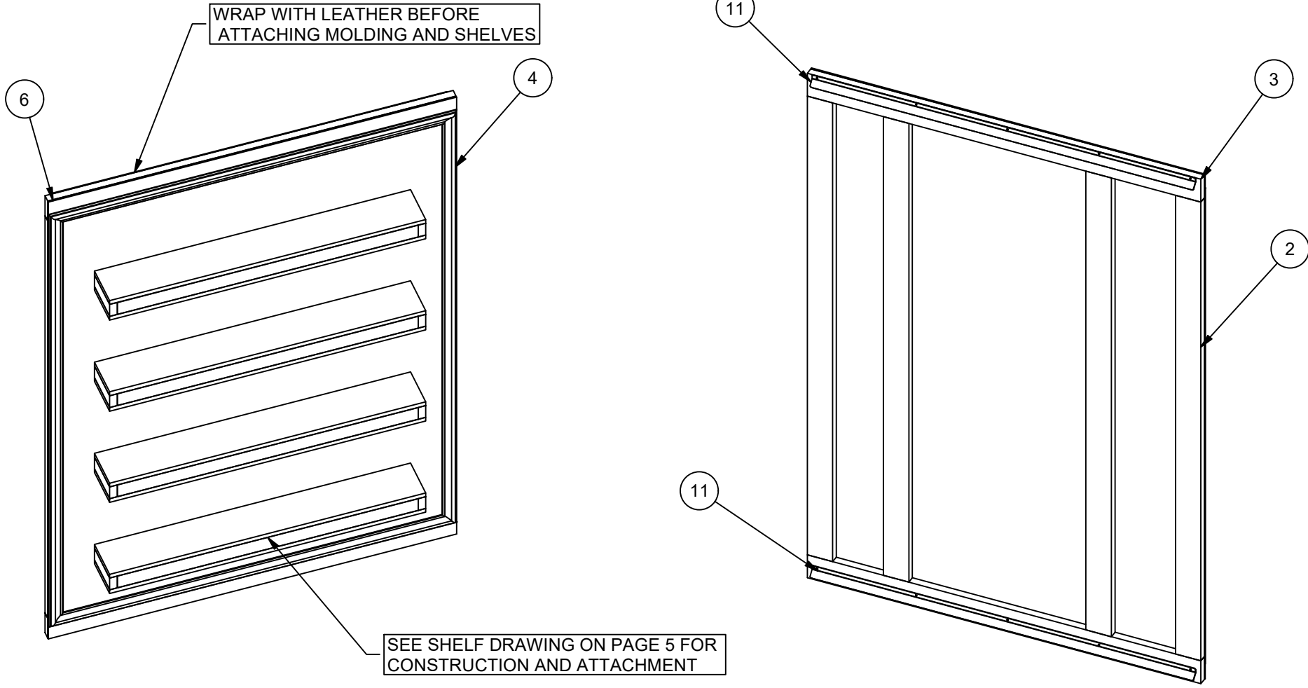
LEFT SHELF COVER B FRONT ISO SCALE 1" = 1'-0"
