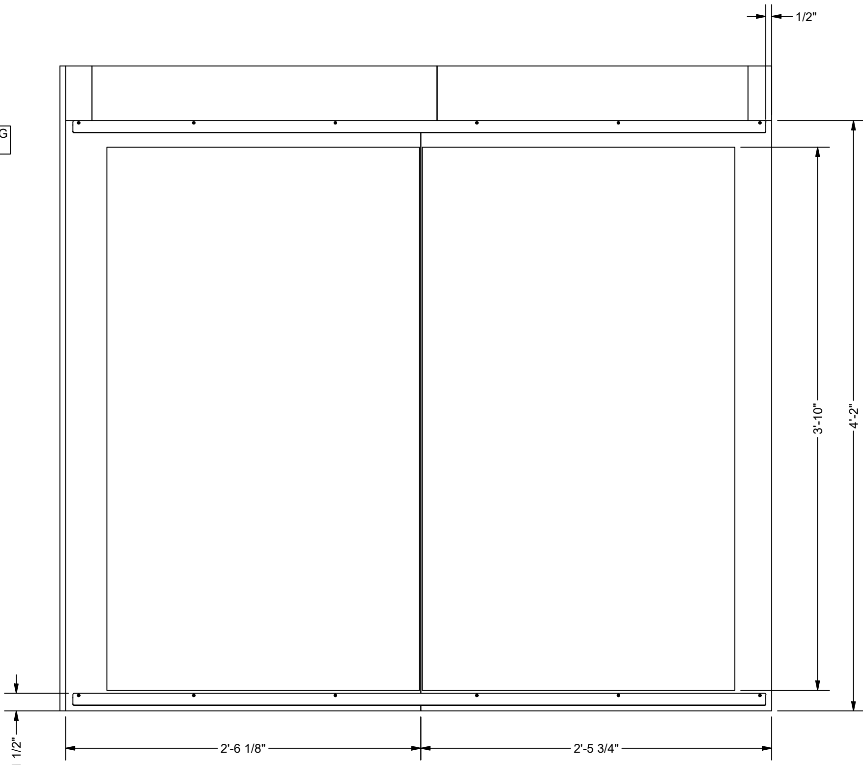
WINDOW COVER BACK SCALE 1 1/2" = 1'-0"
