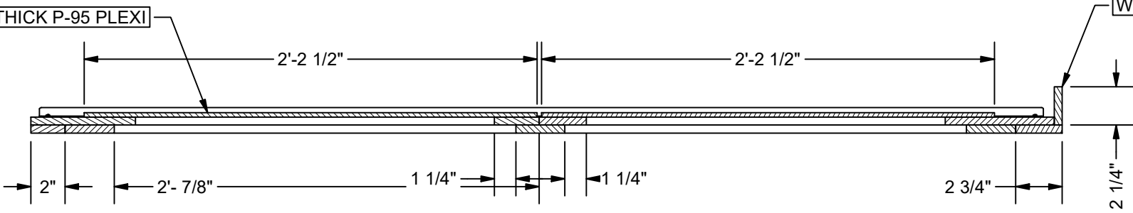
SECTION B-B SCALE 1 1/2" = 1'-0"
