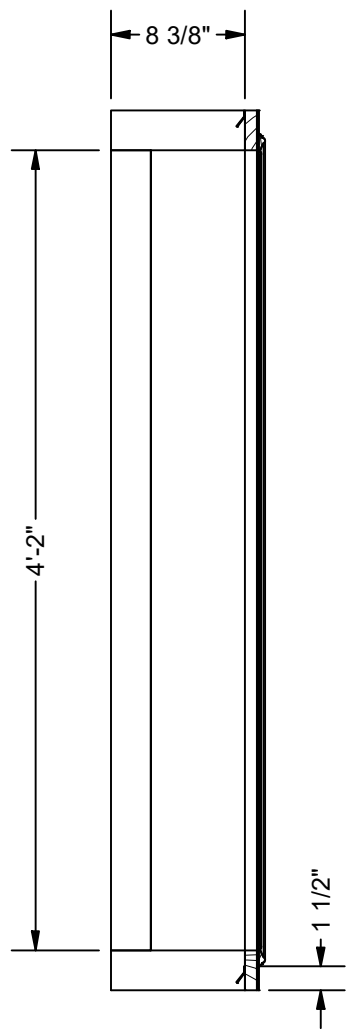
SECTION G-G SCALE 1" = 1'-0"
