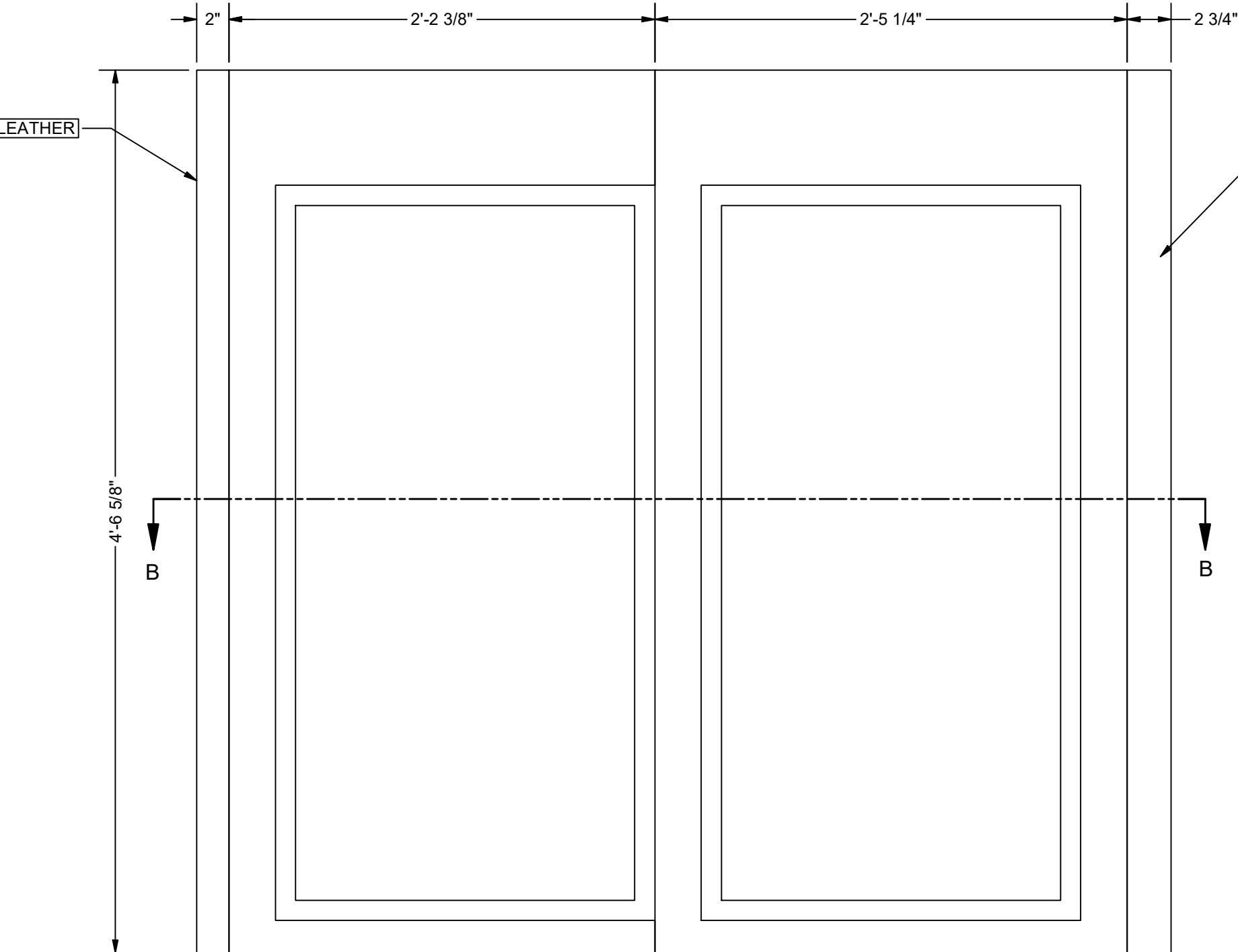
WINDOW COVER FRONT SCALE 1 1/2" = 1'-0"
