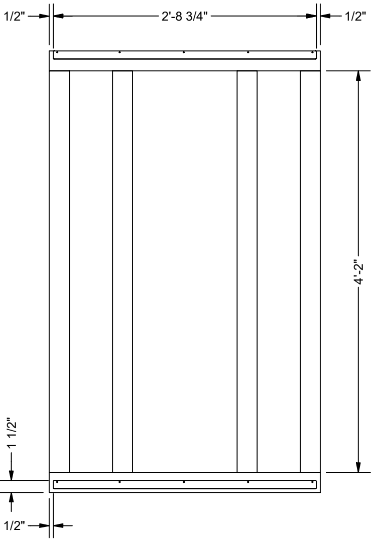
RIGHT SHELF COVER B BACK SCALE 1" = 1'-0"
