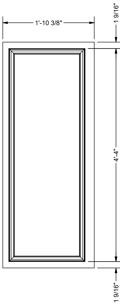
LEFT SHELF COVER C FRONT VIEW SCALE 1" = 1'-0"
