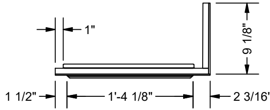
RIGHT SHELF COVER C TOP VIEW SCALE 1" = 1'-0"
