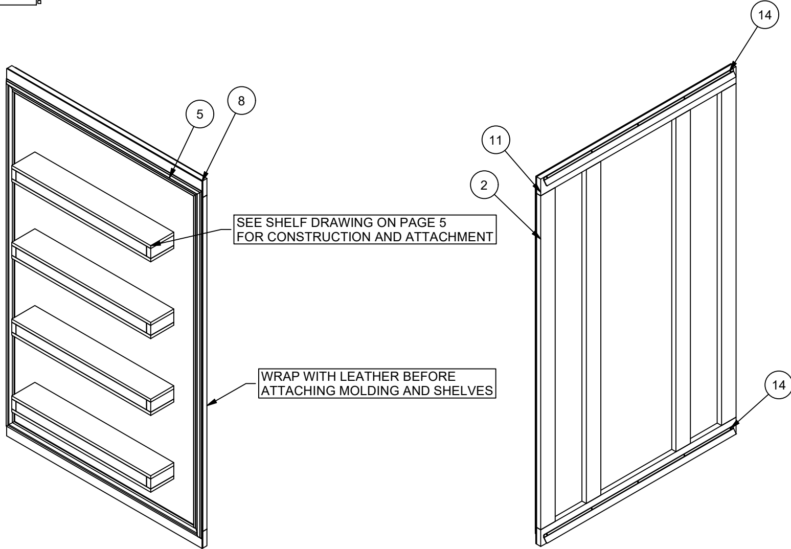
RIGHT SHELF COVER B BACK ISO SCALE 1" = 1'-0"
