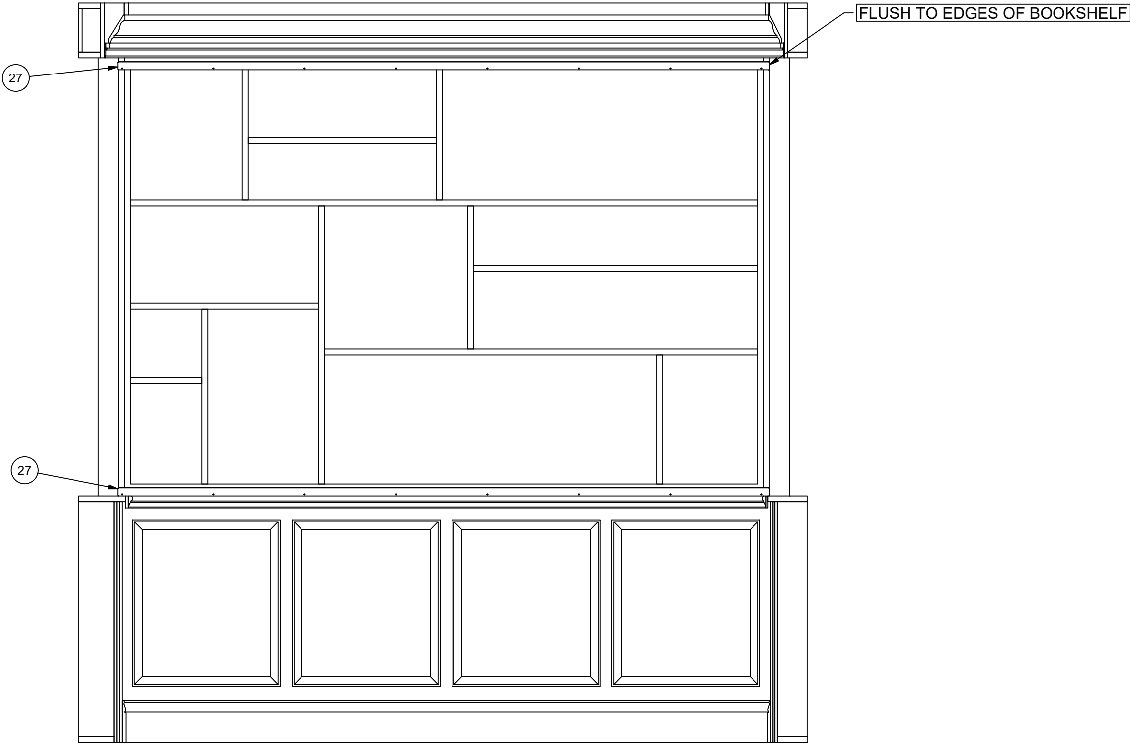
LEFT SHELF SCALE 1" = 1'-0"
