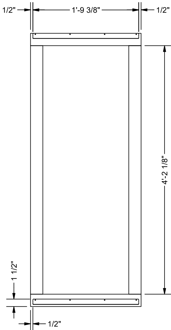
LEFT SHELF COVER A BACK VIEW SCALE 1" = 1'-0"
