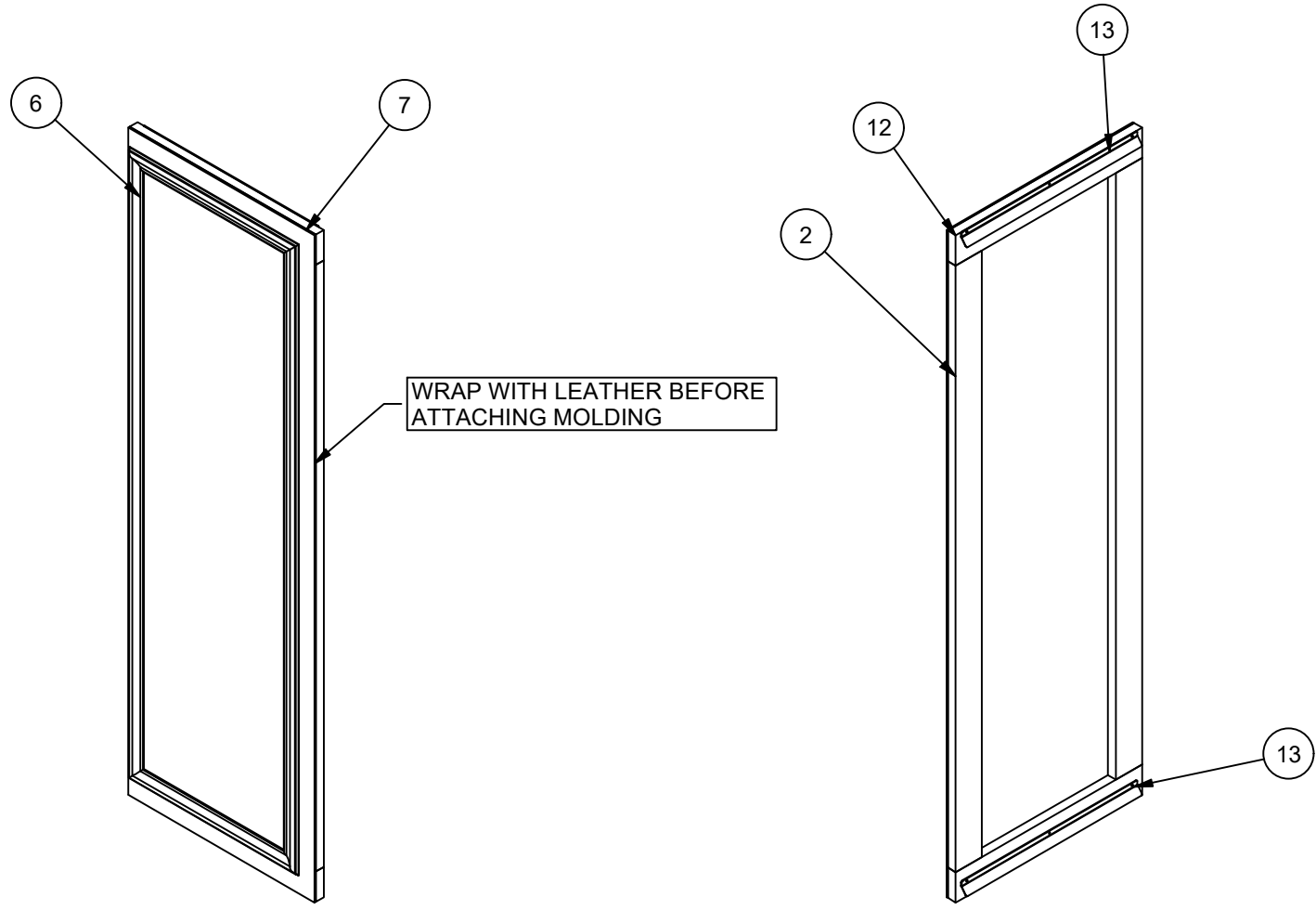
RIGHT SHELF COVER A FRONT ISO SCALE 1" = 1'-0"
