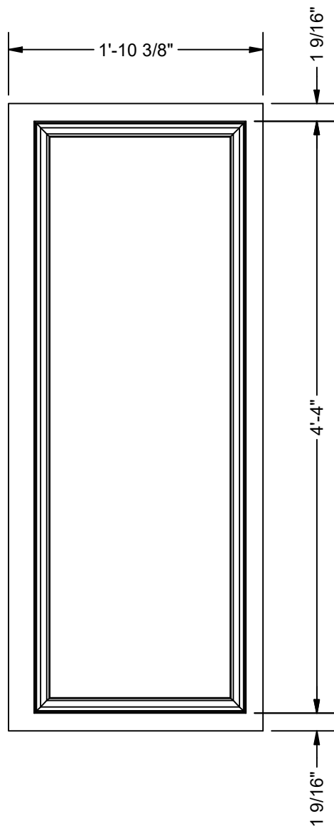
LEFT SHELF COVER A FRONT VIEW SCALE 1" = 1'-0"
