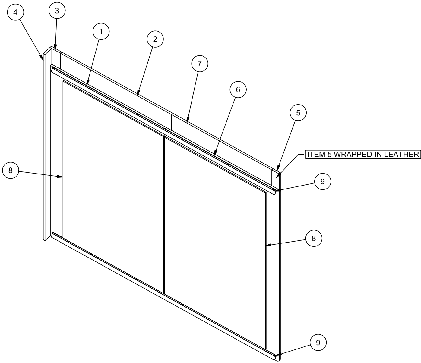
WINDOW COVER BACK ISO SCALE 1" = 1'-0"
