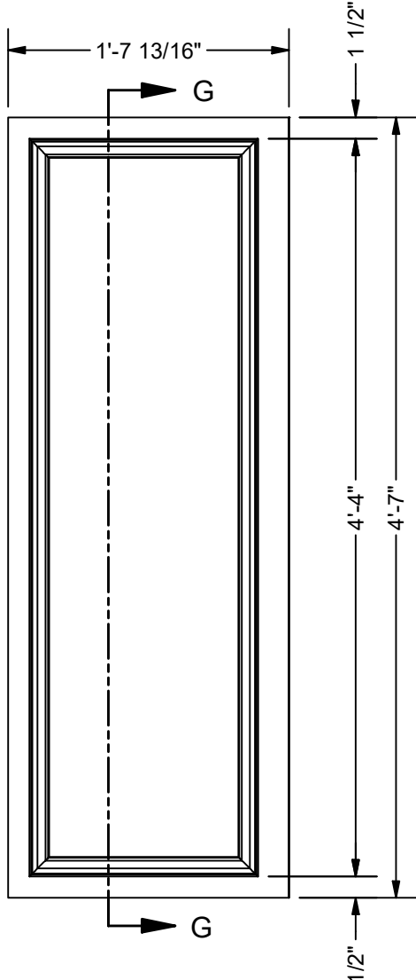
RIGHT SHELF COVER C FRONT SCALE 1" = 1'-0"
