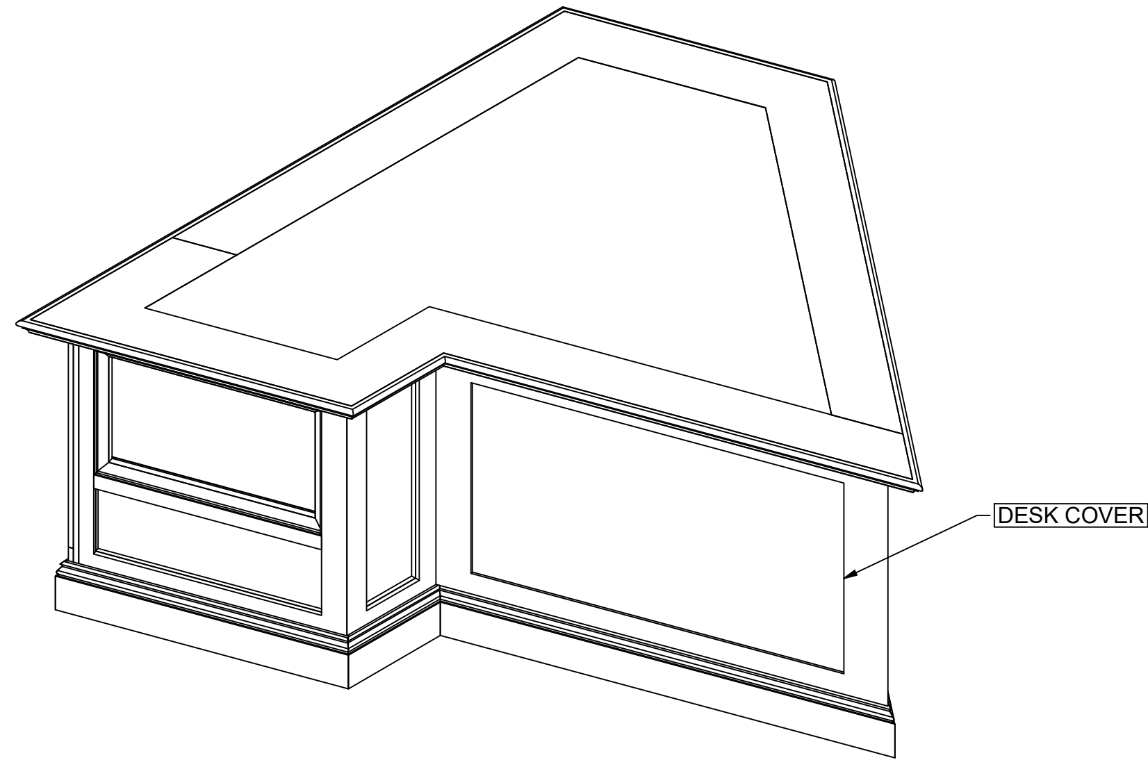
DESK ISO SCALE 1" = 1'-0"
