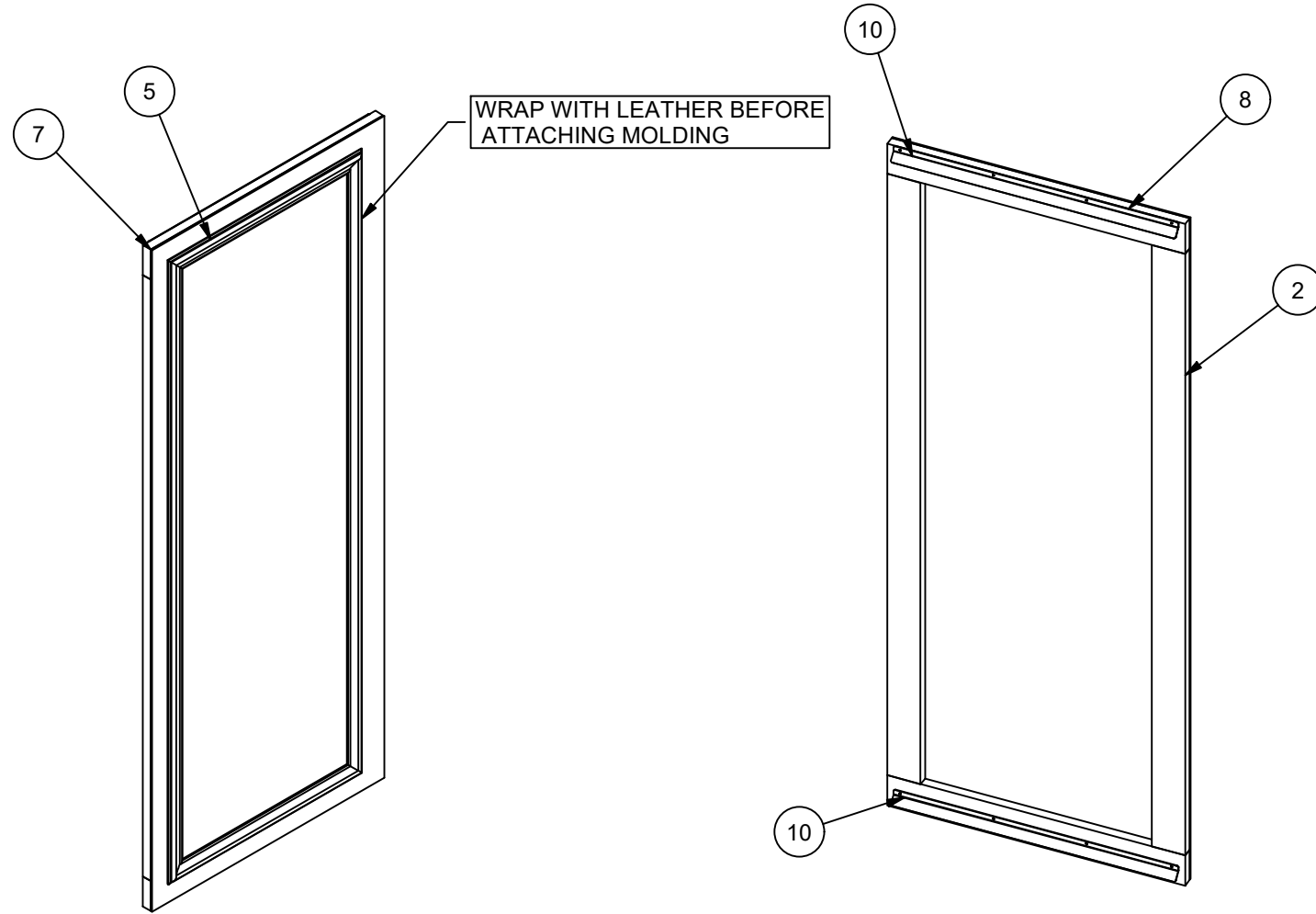
LEFT SHELF COVER C BACK ISO SCALE 1" = 1'-0"
