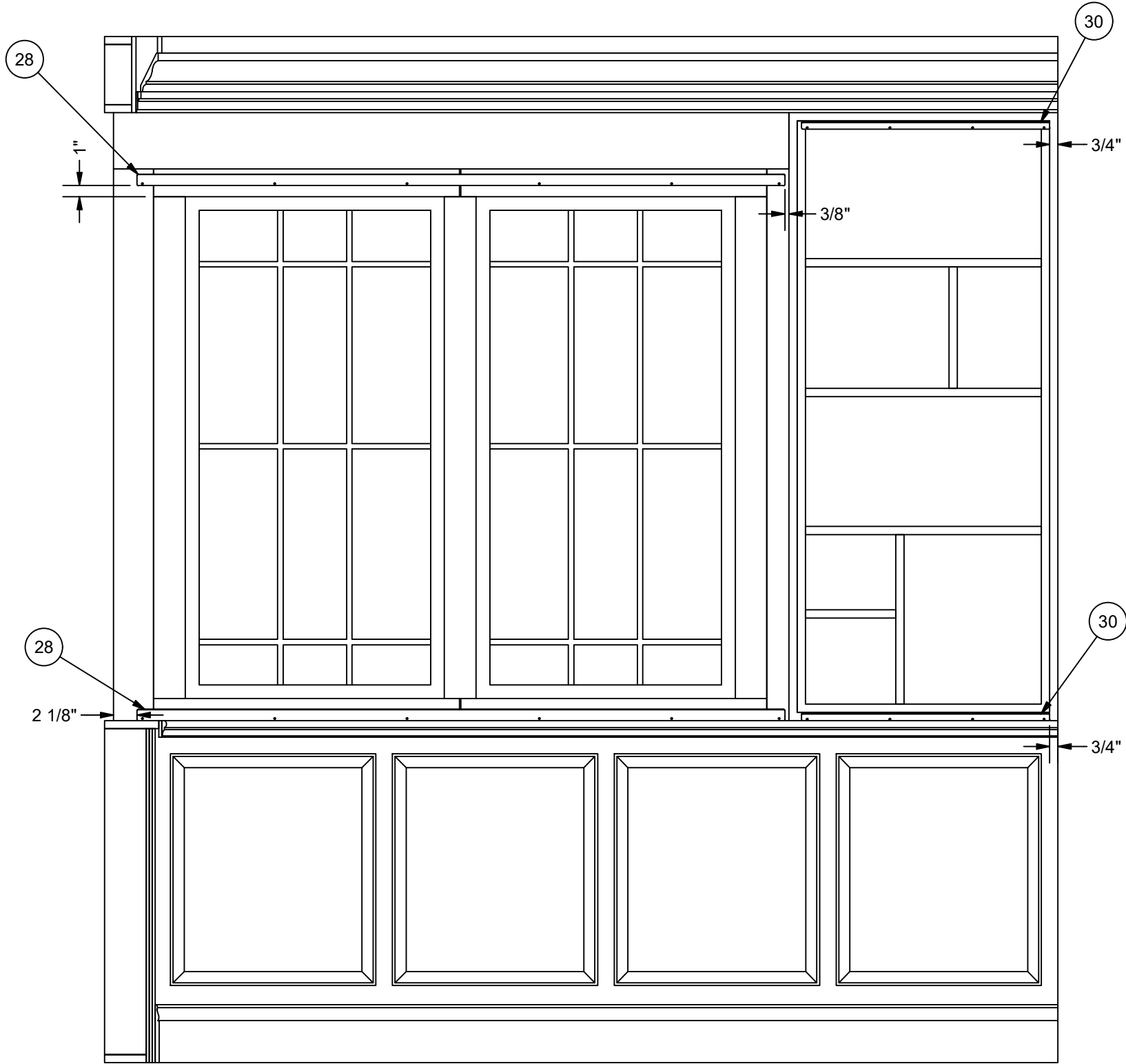
WINDOW WALL SCALE 1" = 1'-0"
