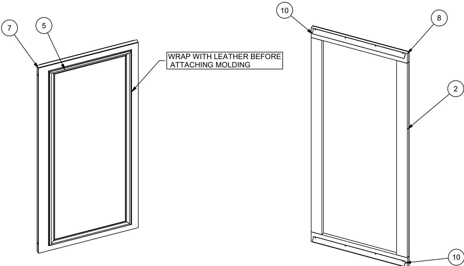
LEFT COVER A BACK ISO SCALE 1" = 1'-0"
