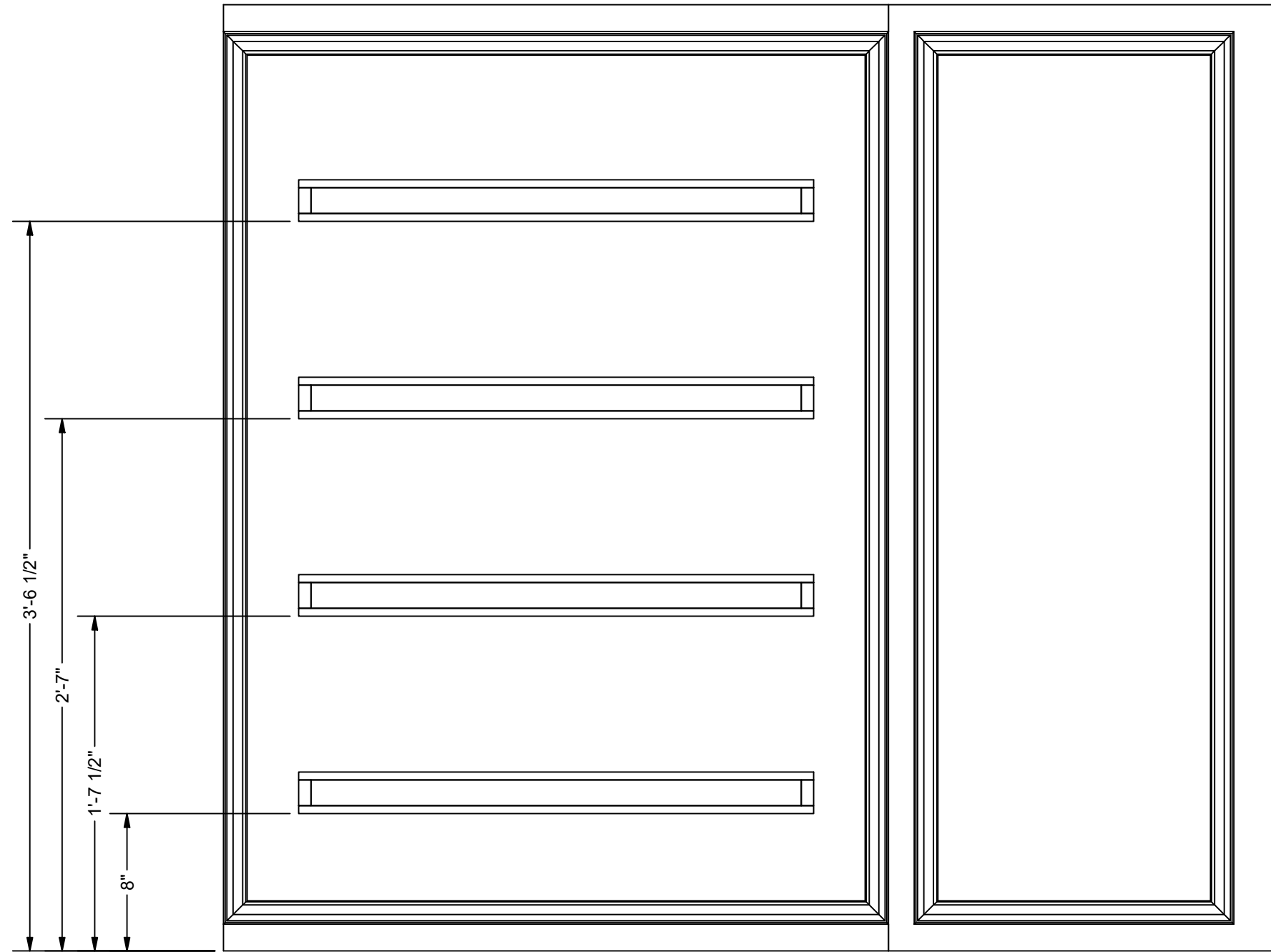
LEFT SHELF PLACEMENT SCALE 1 1/2" = 1'-0"
